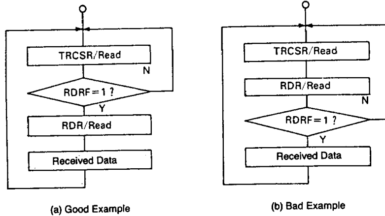
Figure 18 Software polling of SCI-RDRF
