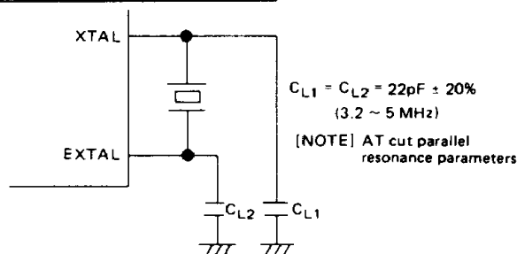
Figure 9 Crystal Interface
