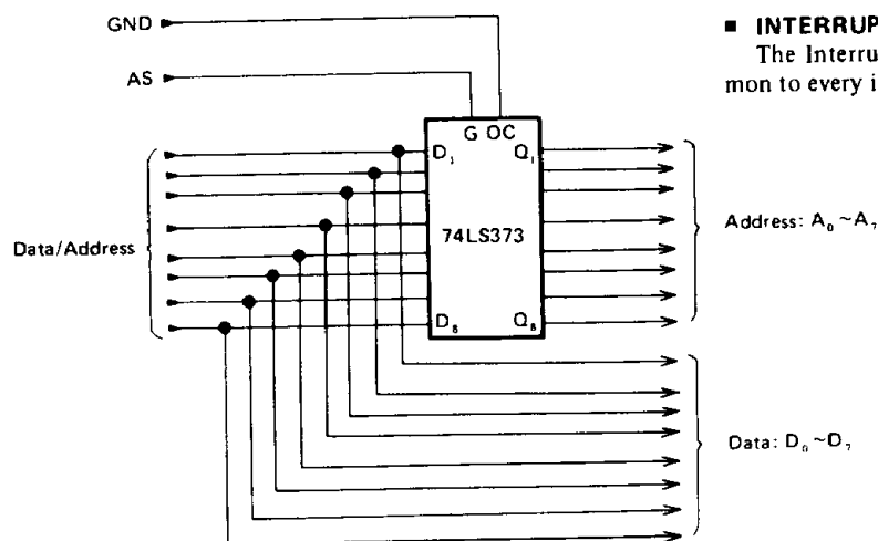
Figure 11 Latch Connection
