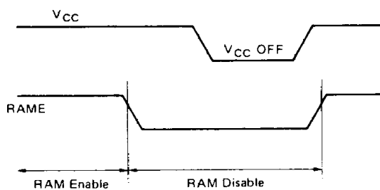
Figure 17 RAM Control Signal (RAME)
