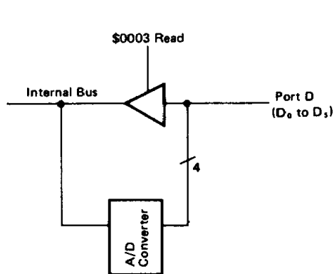
Figure 14 Port D
