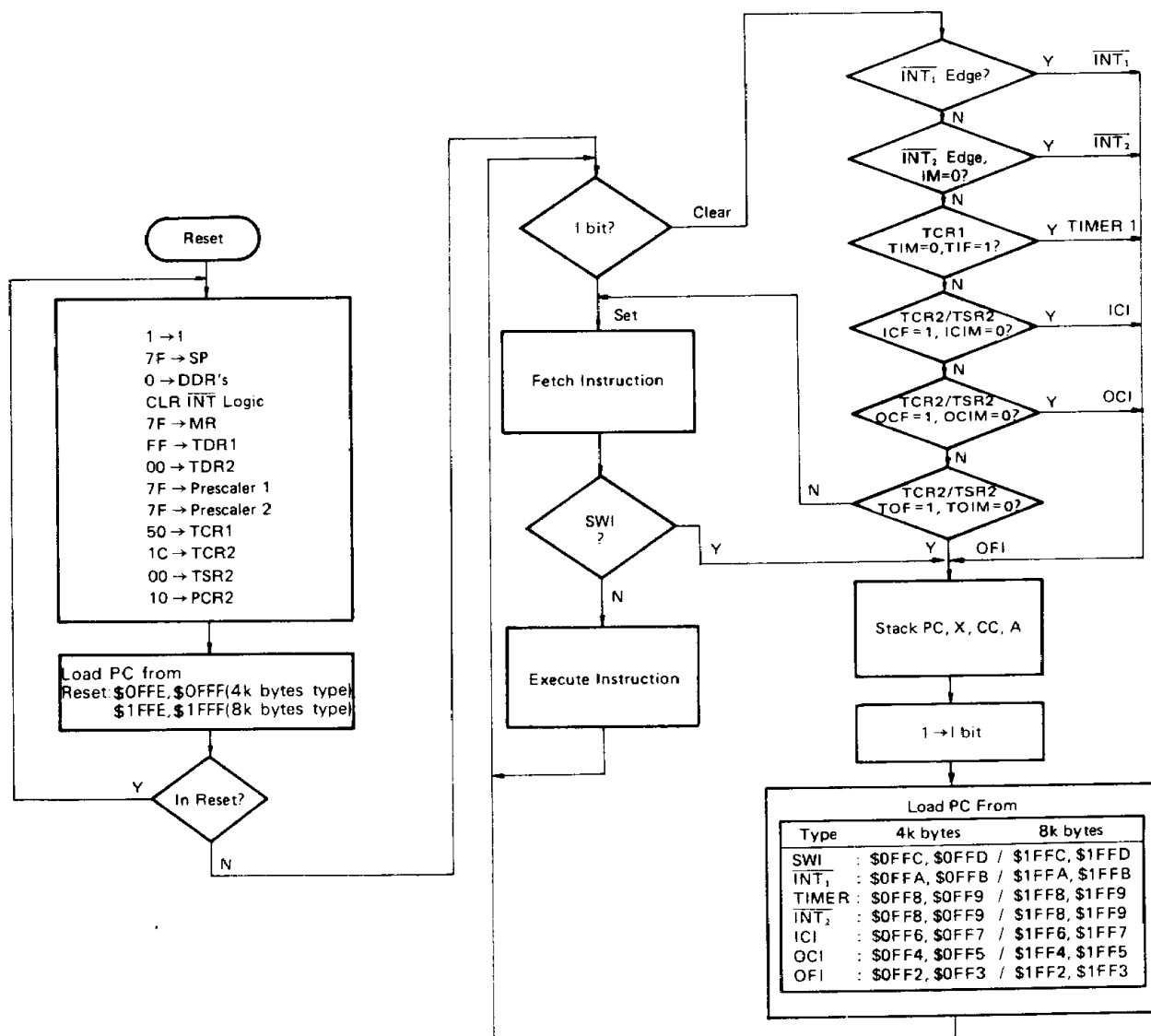
Figure 11 Interrupt Flowchart
