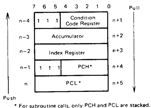
Figure 10 Interrupt Stacking Order
