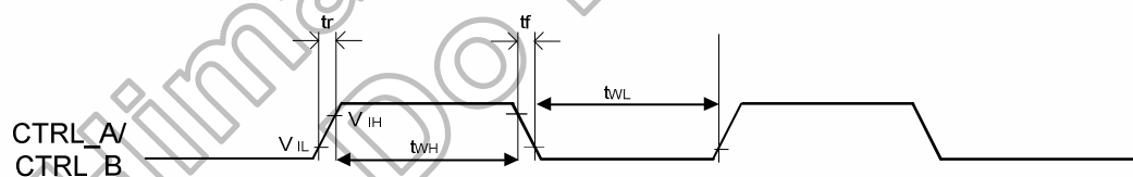
Figure 12.2: Control signal timing characteristics
