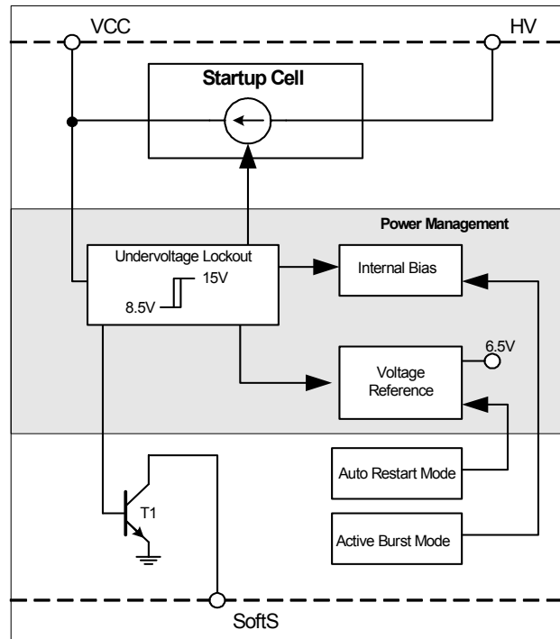
Figure 4 Power Management
