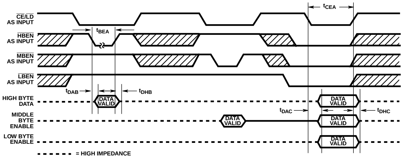
FIGURE 4. DIRECT MODE TIMING DIAGRAM
