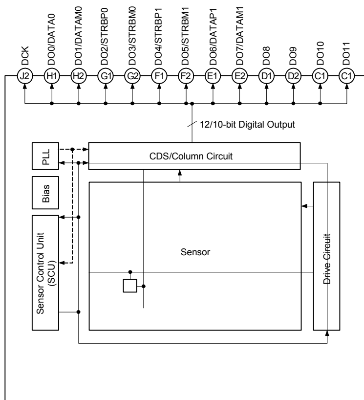
Block Diagram
