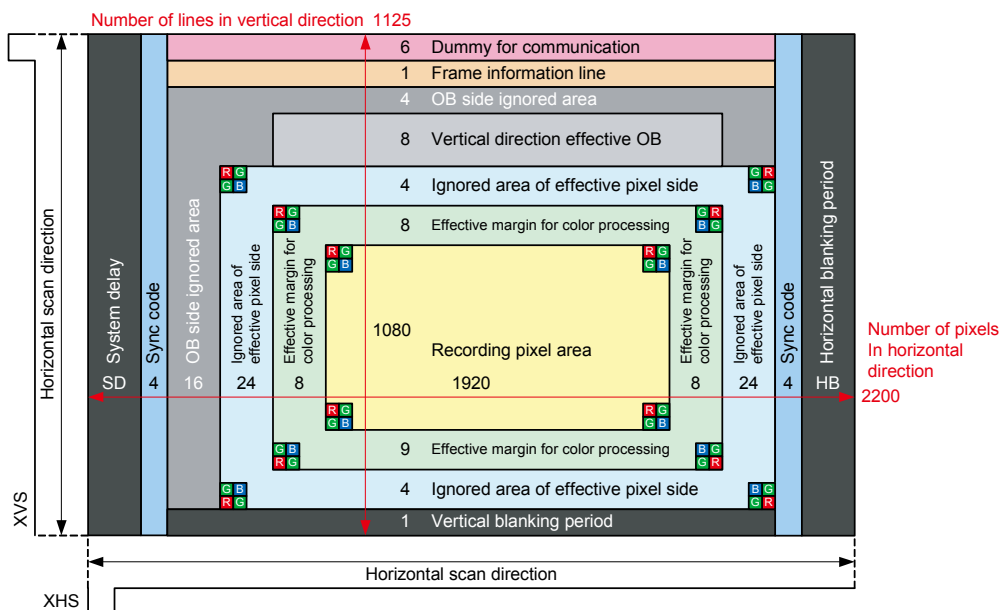
Pixel Array Image Drawing in HD1080 p Mode
