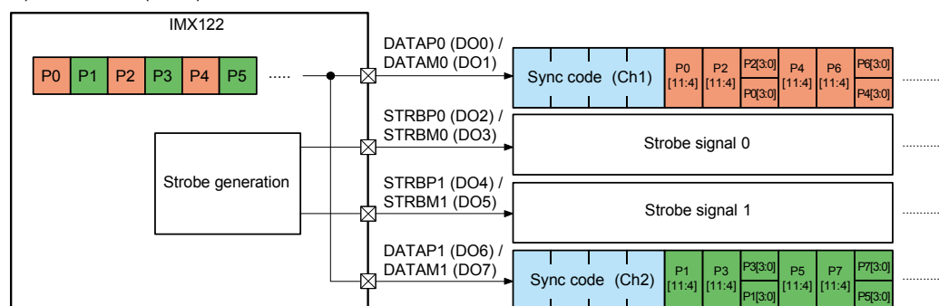
C) 2ch-RAW12 (12 bit)
