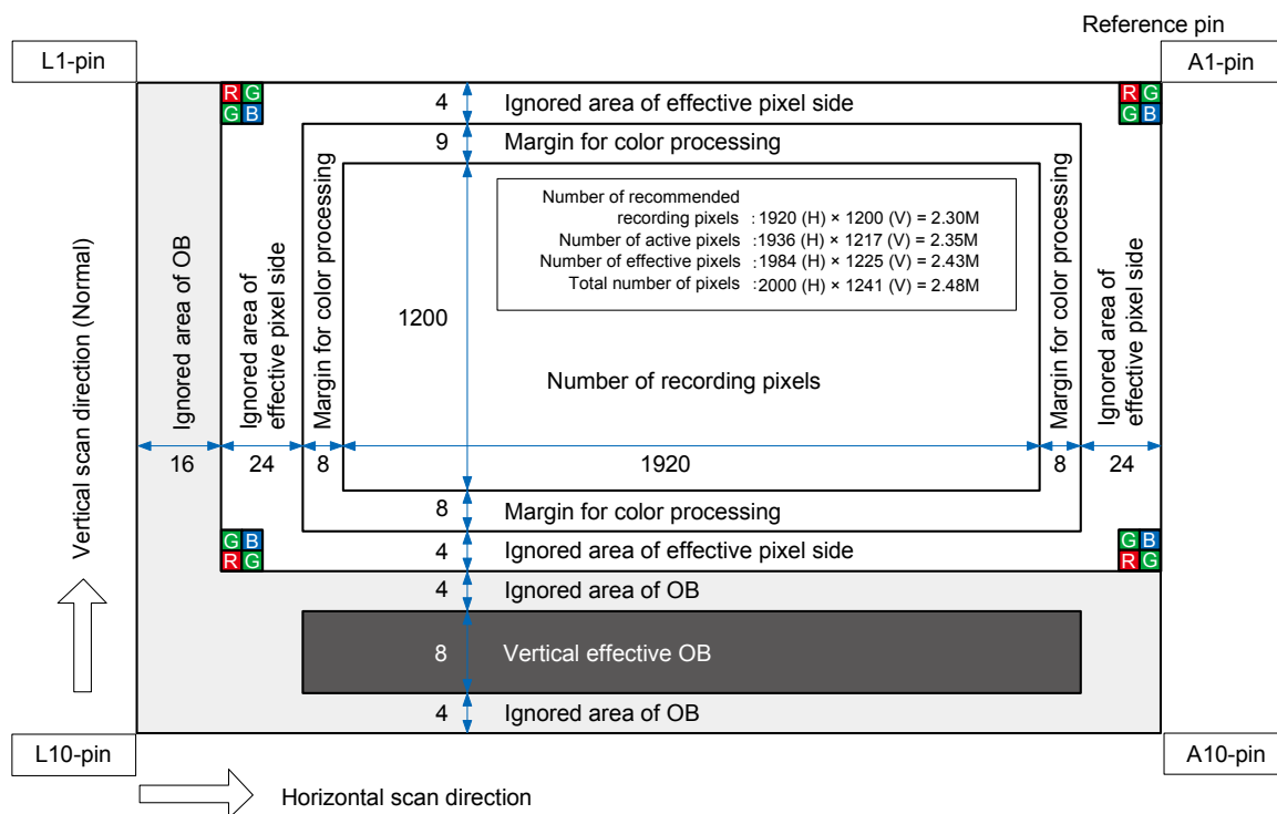
Pixel Arrangement - Physical Image
