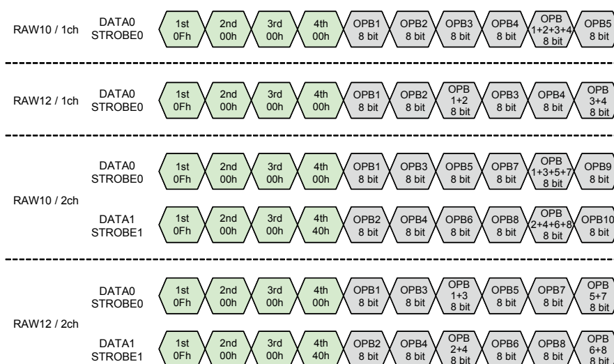
Example of Sync Code Output
