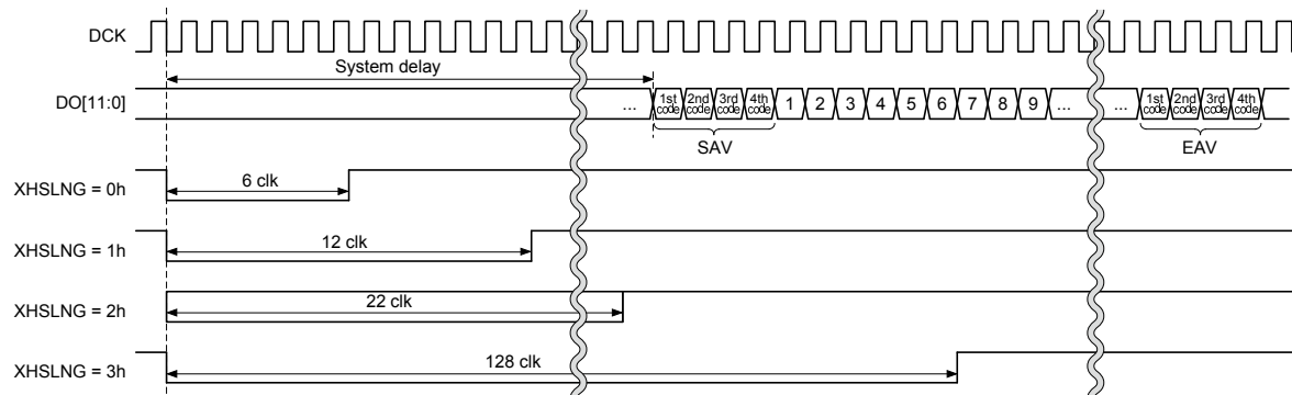
List of XHS Pulse Width Setting
