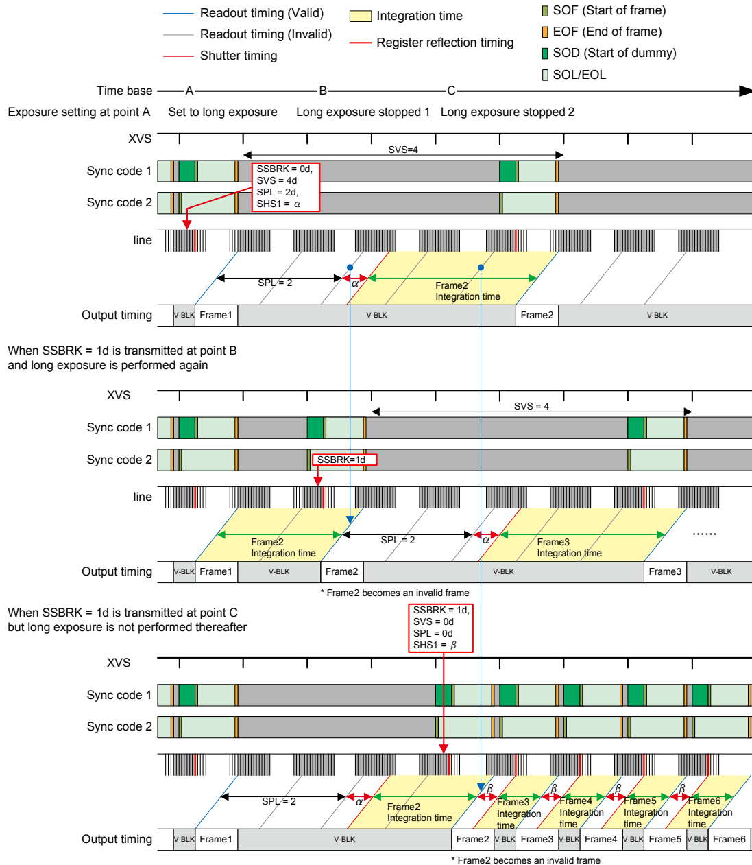
Example Showing Application of the Shutter Break Function
