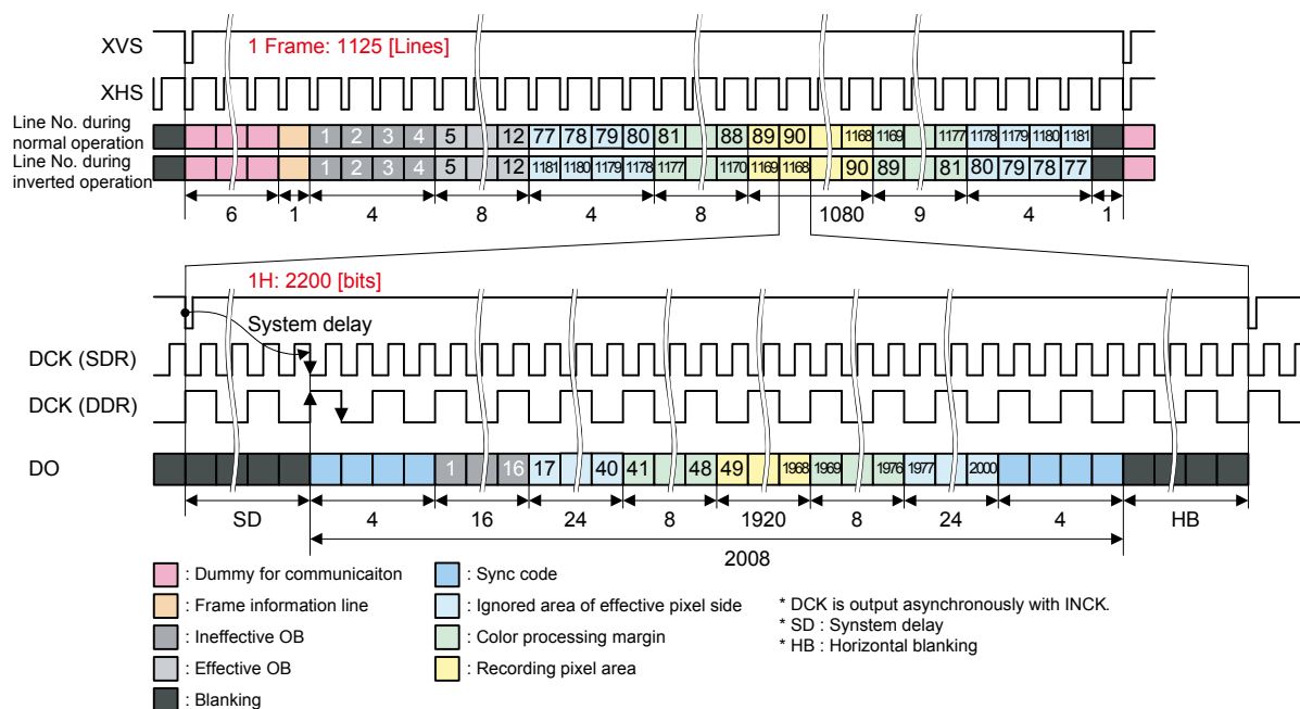
Drive Timing Chart for Parallel CMOS Output in HD1080 p Mode
