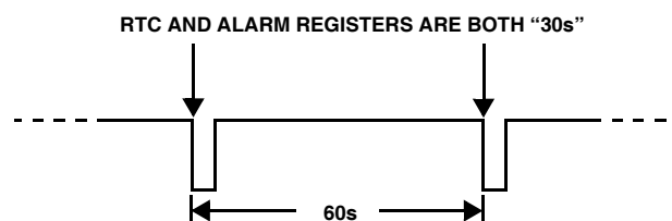
FIGURE 5. \overline{\text{IRQ}} WAVEFORM
