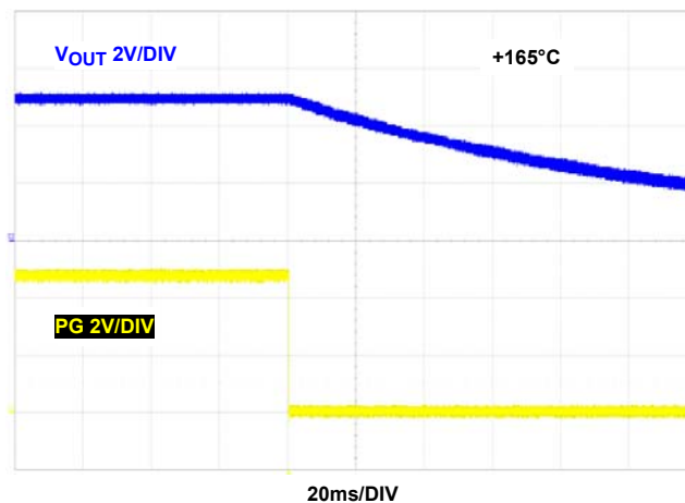
FIGURE 40. OVER-TEMPERATURE PROTECTION
