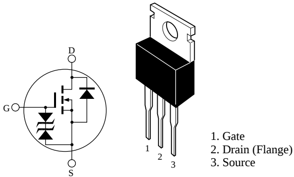
TO-220AB
