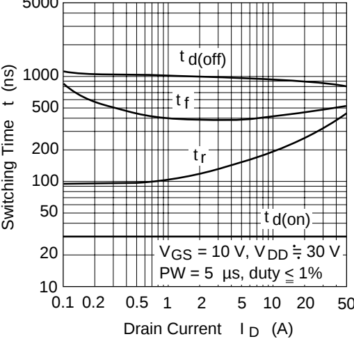
Switching Characteristics
