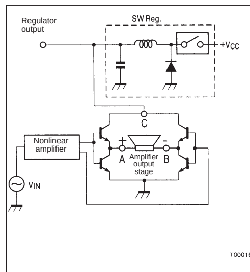
Figure 1 Overview Block Diagram
