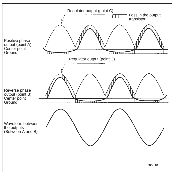
Figure 3 Output Waveforms
