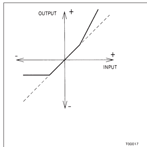
Figure 2 Nonlinear Amplifier Input/Output Characteristics
