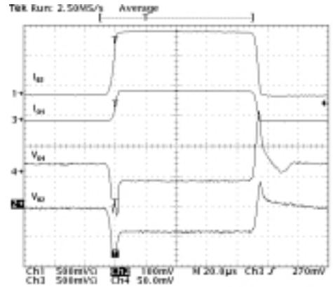
Figure 25: Load Transient
