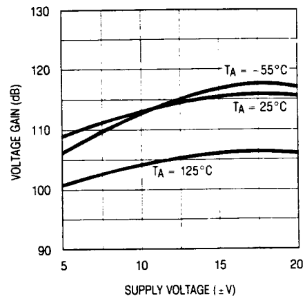
Voltage Gain
