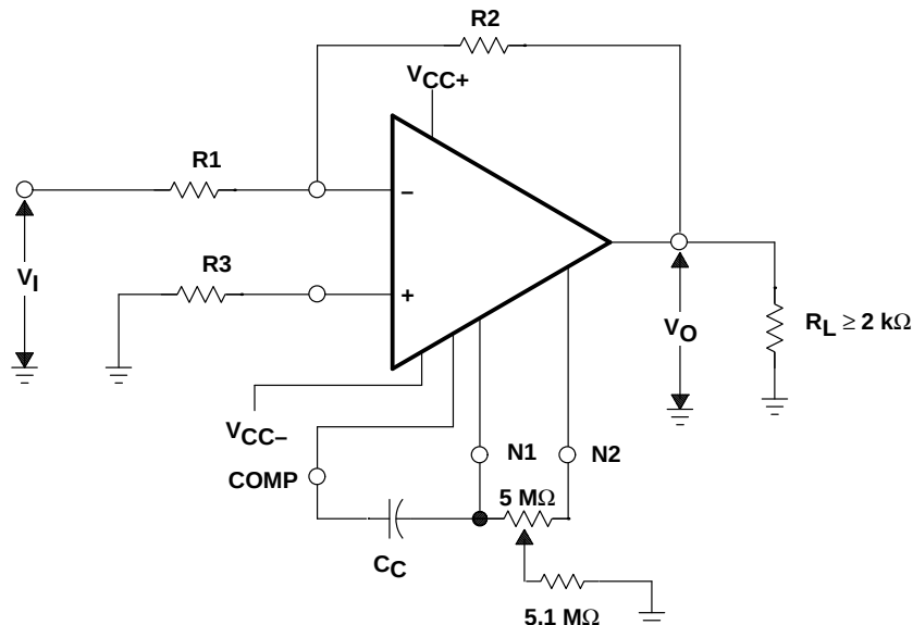
Figure 7. Inverting Circuit with Adjustable Gain, Single-Pole Compensation, and Offset Adjustment
