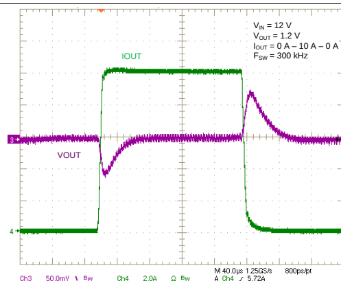
Figure 16. 10-A Step Load Transient Response, 2.5-A/μs Slew Rate
