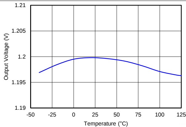
Figure 5. Temperature Regulation
