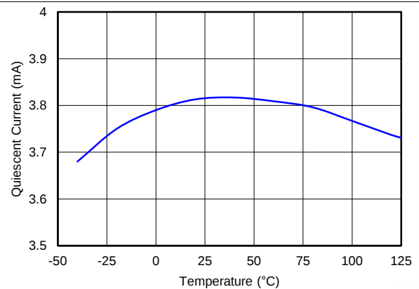
Figure 6. Quiescent Current vs. Temperature, Nonswitching
