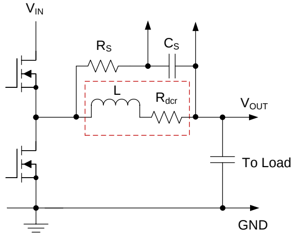
Figure 30. Current Sensing Using Inductor DCR
