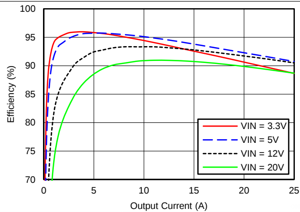
Figure 1. Efficiency Plot, V_{OUT} = 1.2\text{ V}
