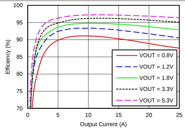
Figure 2. Efficiency Plot, V_{IN} = 12\text{ V}
