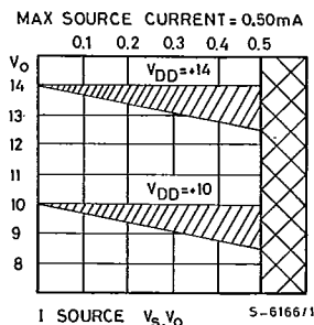
Fig. 2 - Output signal d.c. loading
