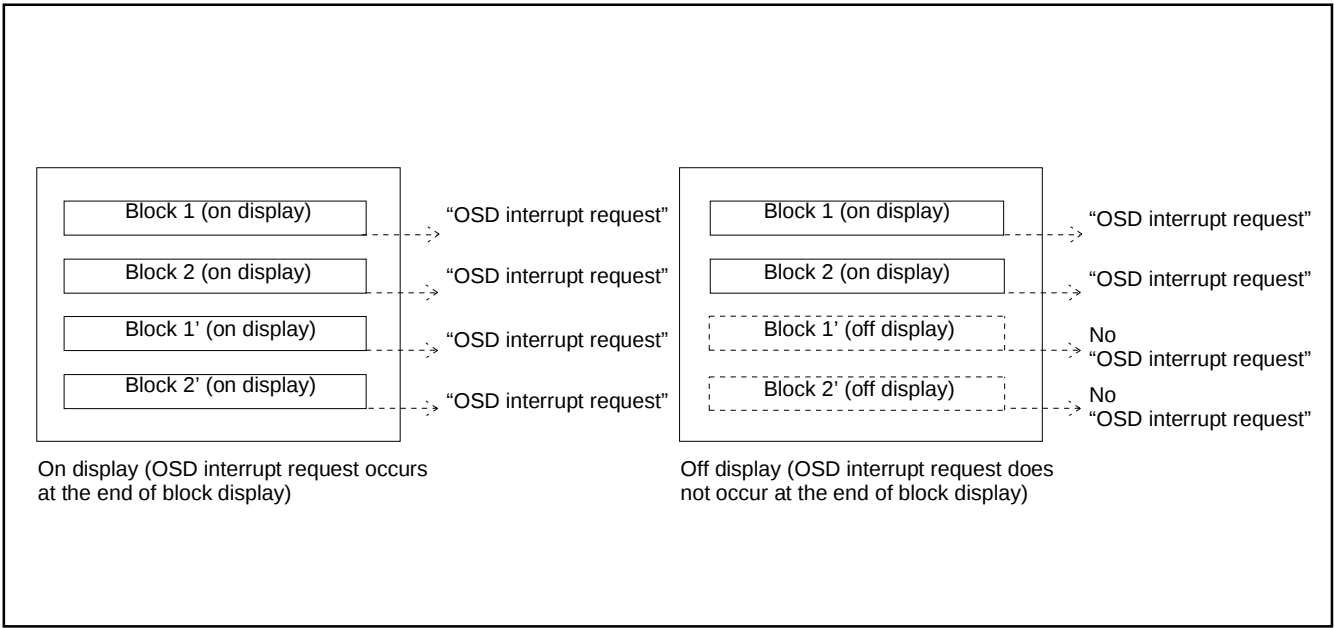
Fig. 8.10.16 Note on Occurence of OSD Interrupt
