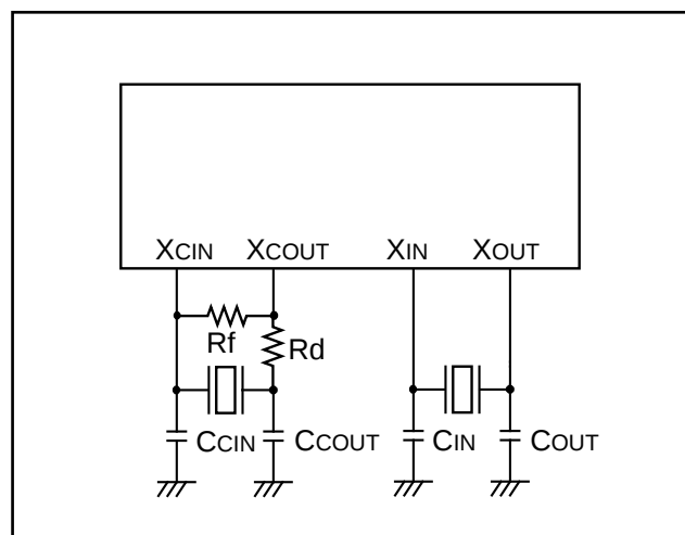
Fig. 55. Ceramic resonator circuit
