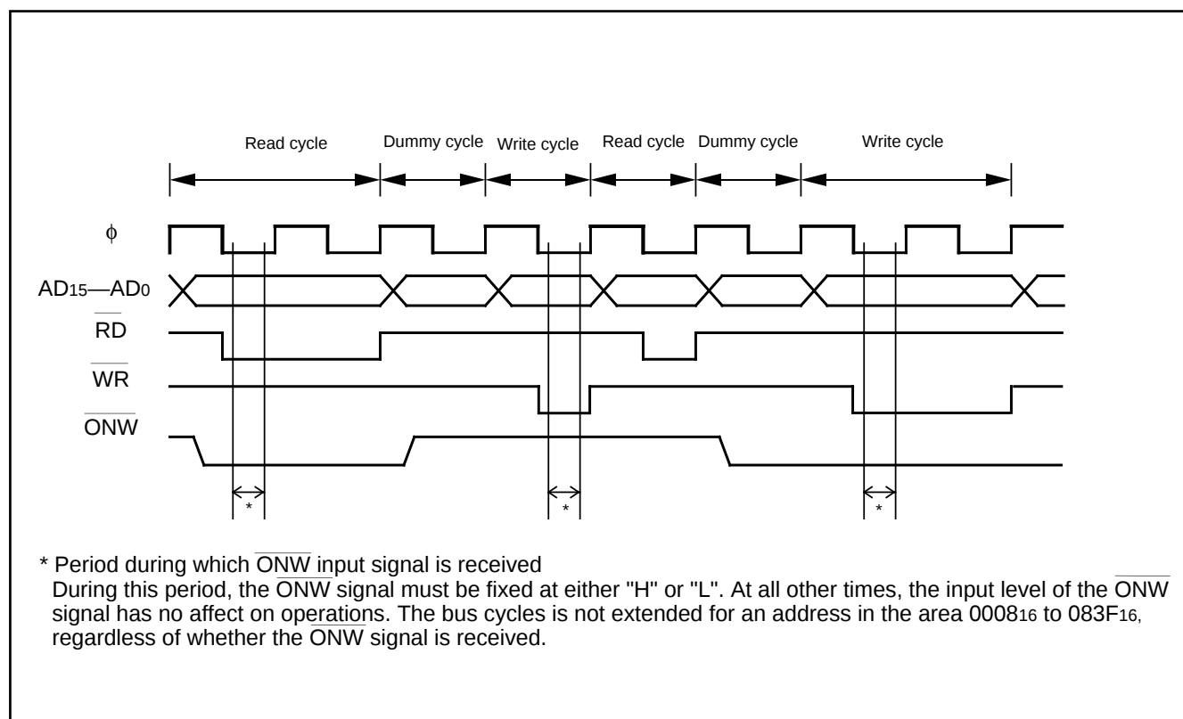
Fig. 61. \overline{\text{ONW}} function timing
