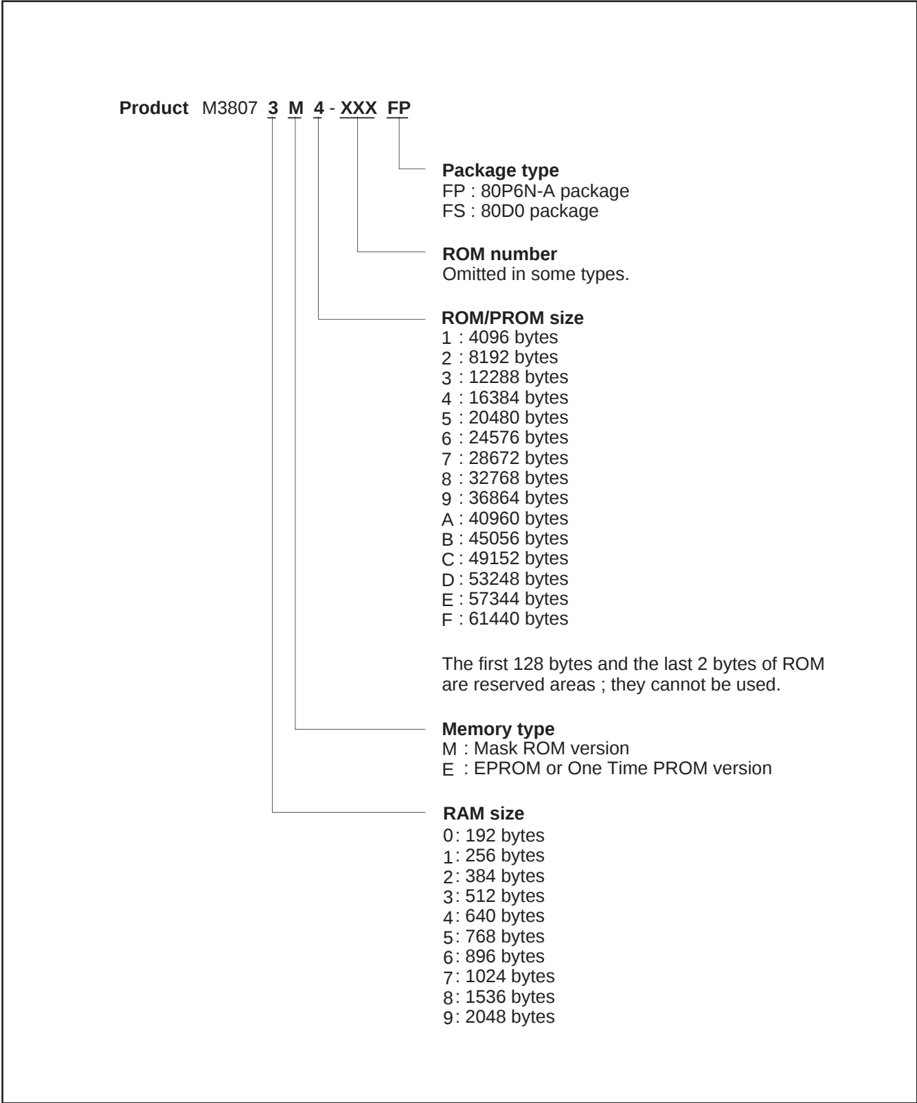
Fig. 3. Part numbering
