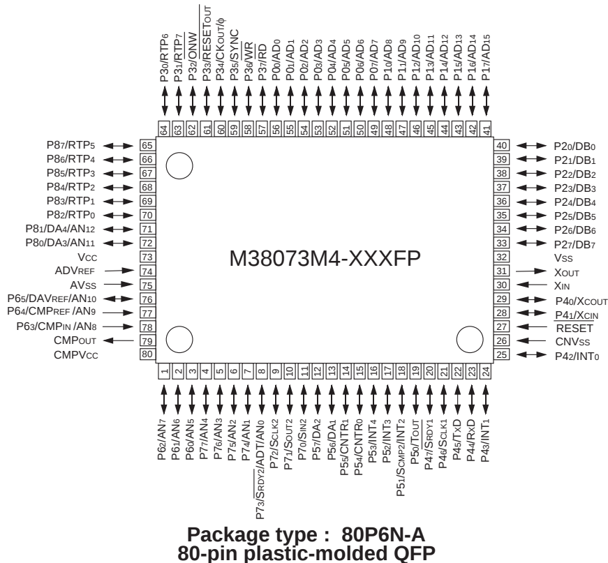
Fig. 1. Pin configuration of M38073M4-XXXXP
