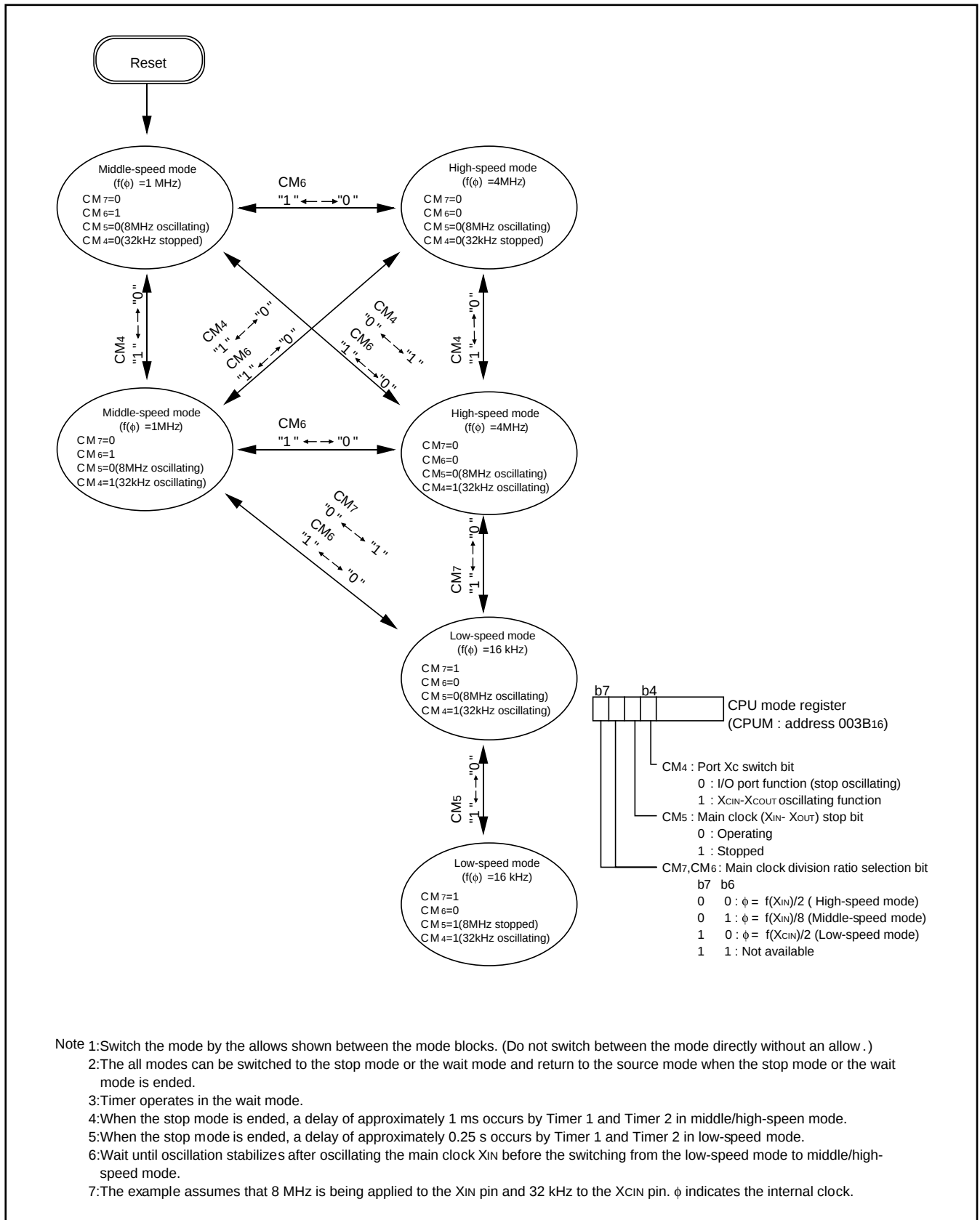
Fig. 58. State transitions of system clock
