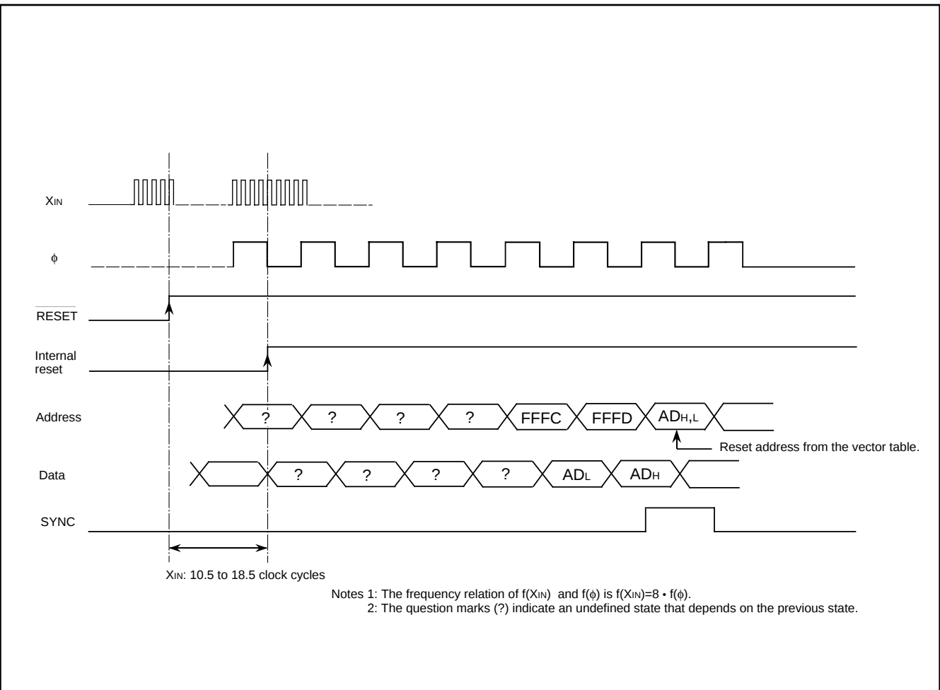
Fig. 53. Reset sequence
