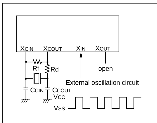
Fig. 56. External clock input circuit
