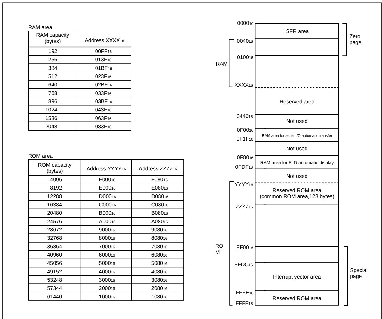
Fig. CA-1 Memory map
