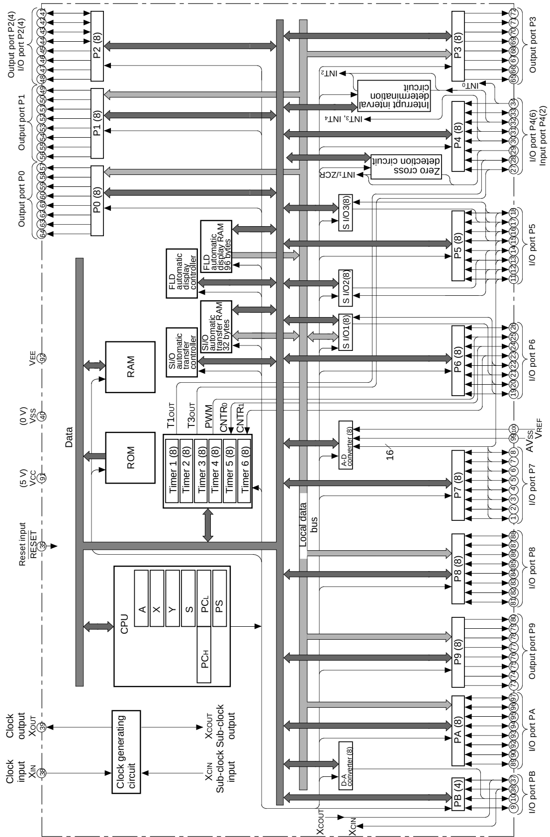
FUNCTIONAL BLOCK DIAGRAM (Package : 100P6S-A)
