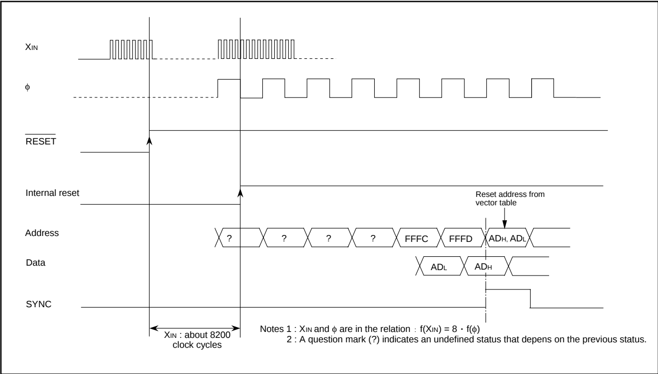
Fig. 34 Reset sequence
