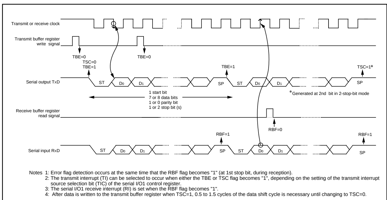
Fig. 18 Operation of UART serial I/O1 function
