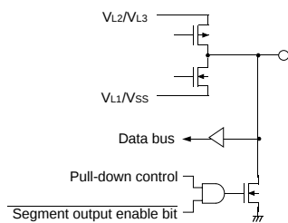
(3) Ports P30-P37
