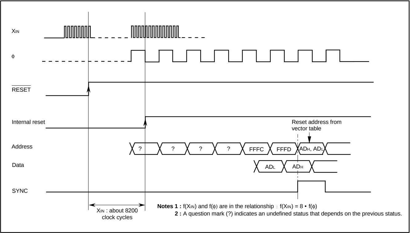
Fig. 31 Reset sequence
