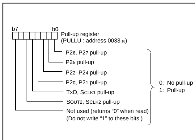
Fig.11 Structure of Pull-up Register
