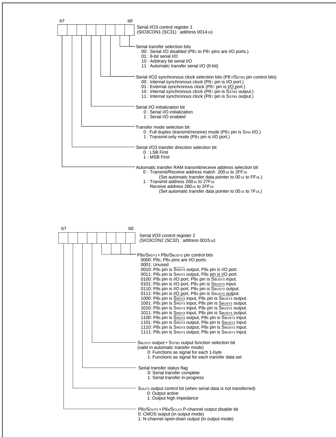
Fig. 35 Structure of serial I/O3 control registers 1 and 2
