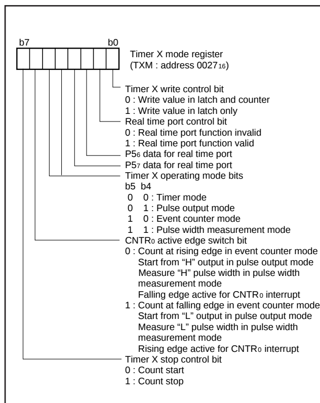
Fig. 23 Structure of timer X mode register
