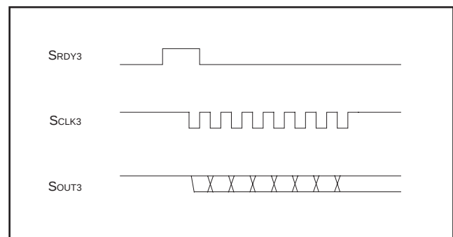
Fig. 48 SRDY3 Input Operation (internal synchronous clock)
