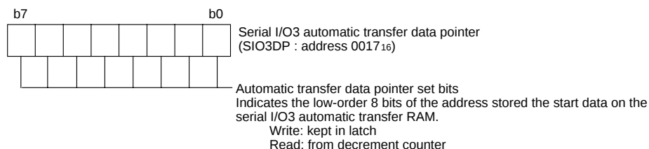
Fig. 37 Structure of serial I/O3 automatic transfer data pointer
