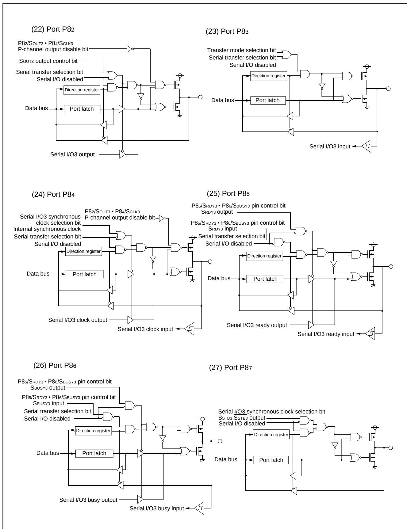
Fig. 16 Port block diagram (5)
