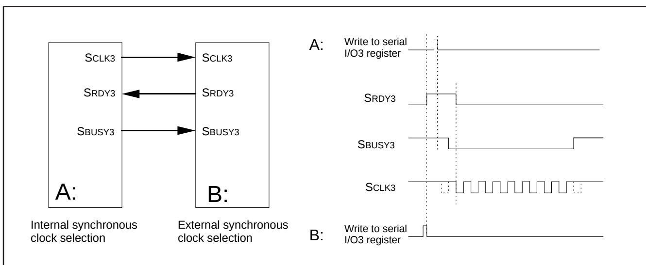
Fig. 50 Handshake operation at serial I/O3 mutual connecting (2)
