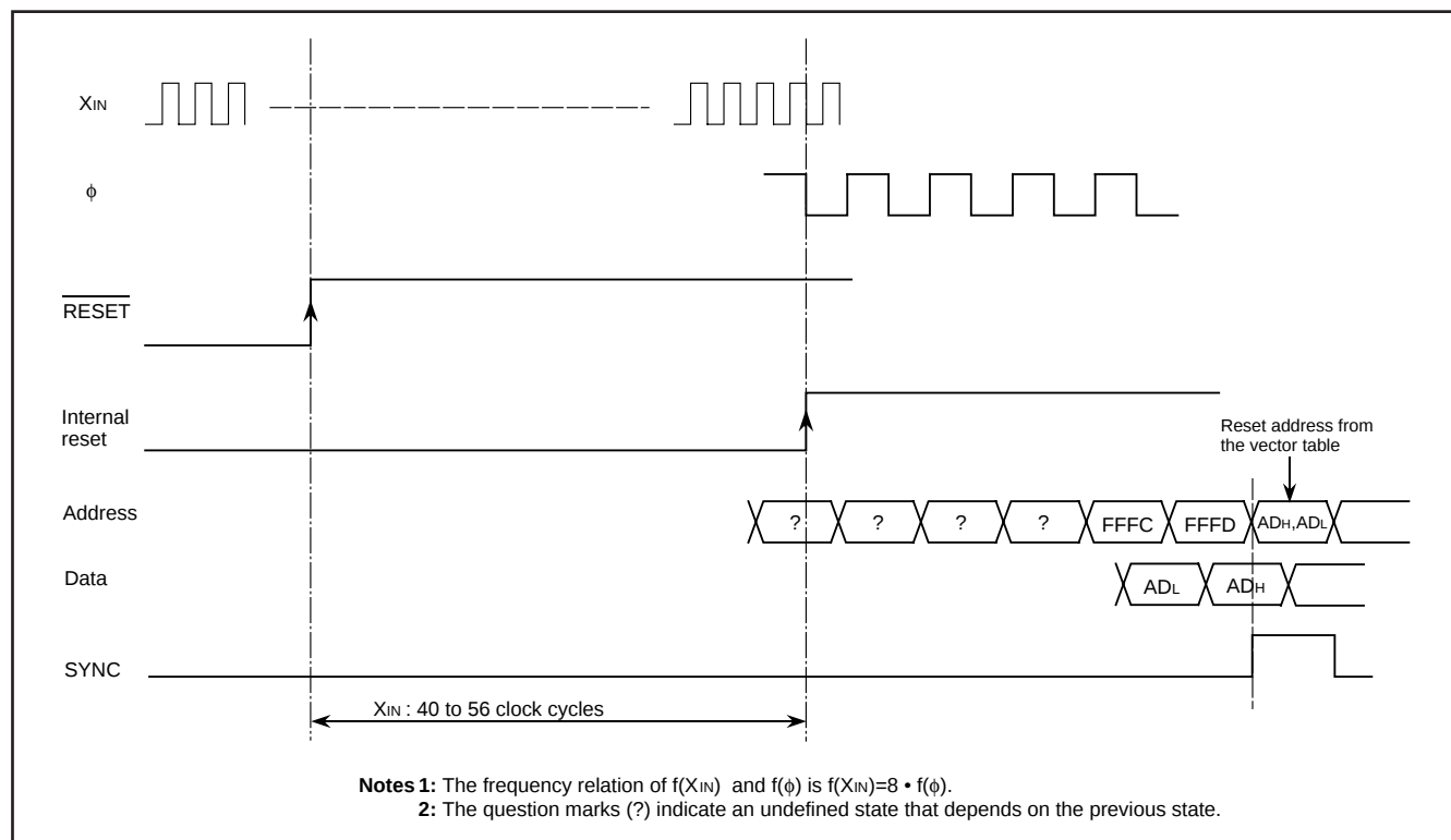
Fig. 66 Reset sequence
