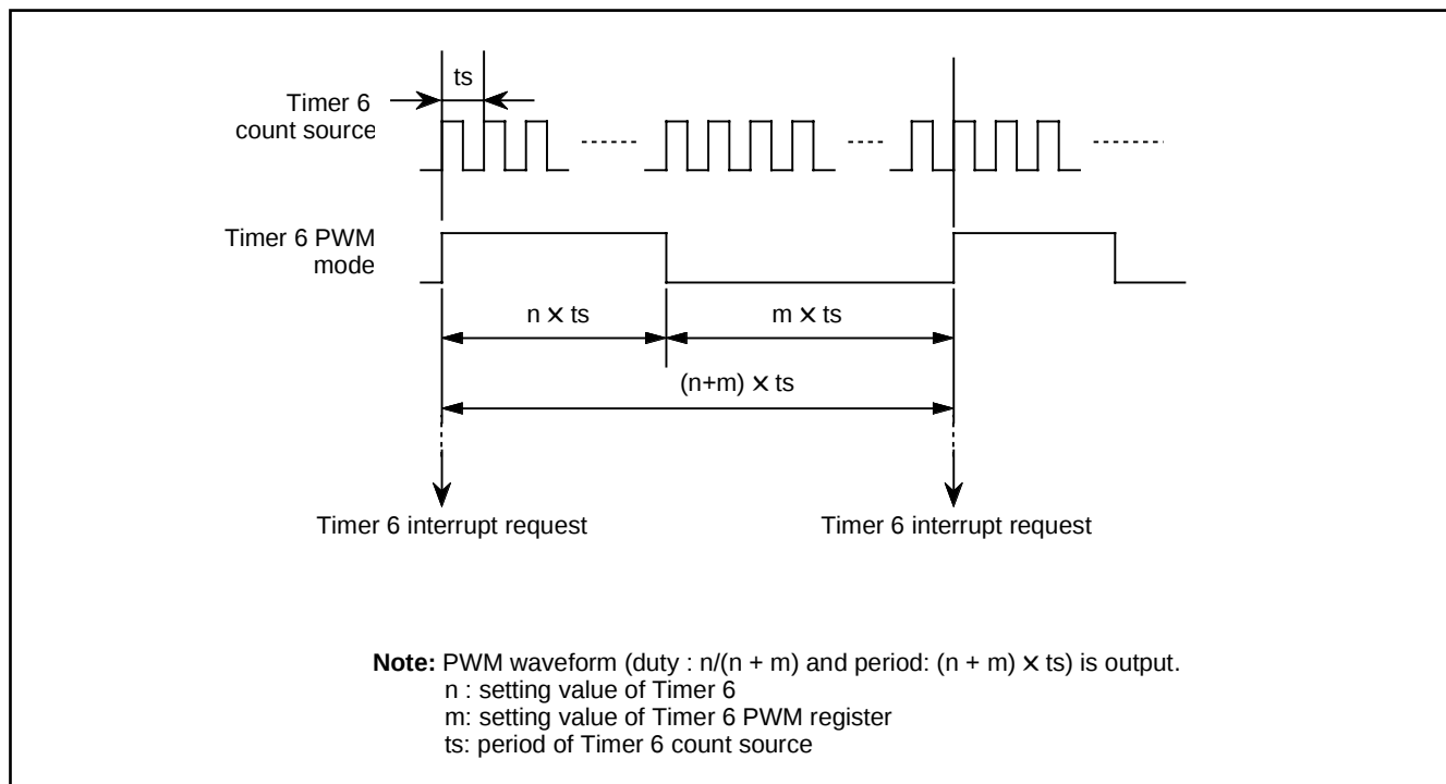
Fig. 19 Timing chart of timer 6 PWM 1 mode
