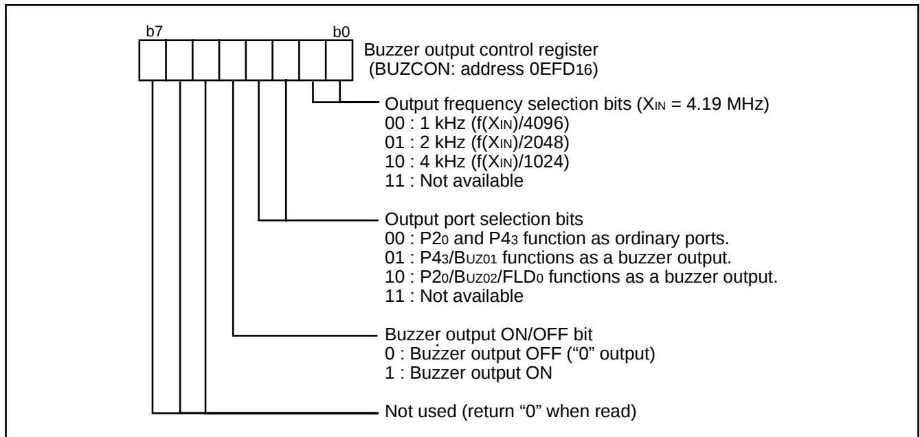
Fig. 67 Structure of buzzer output control register
