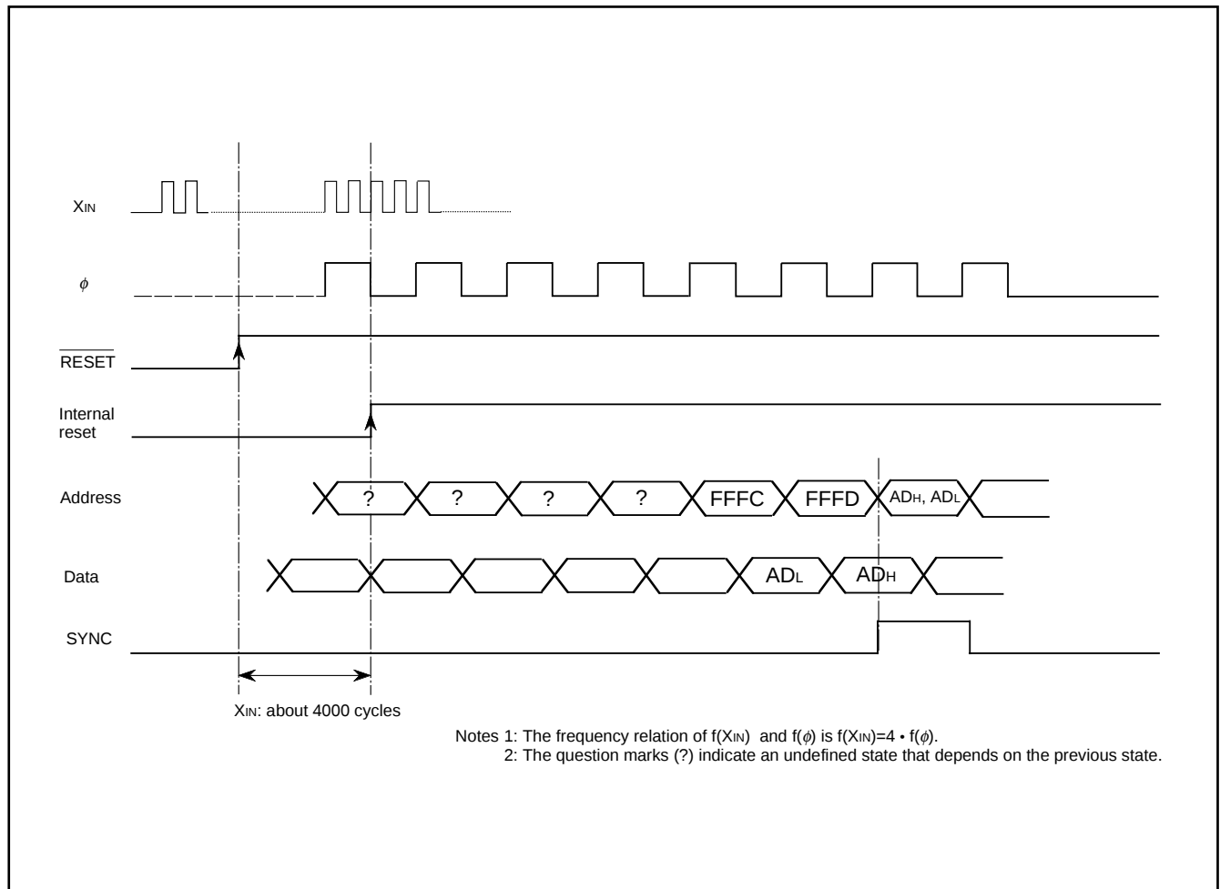
Fig. 69 Reset sequence
