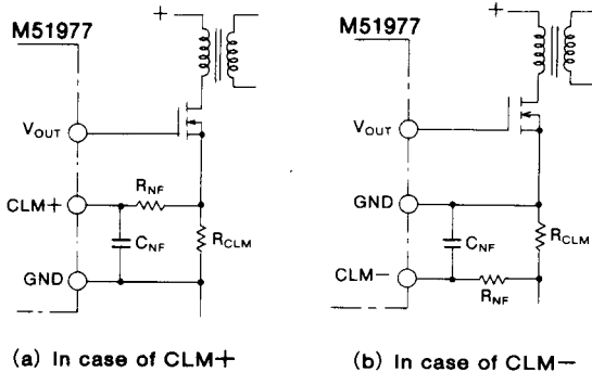
Fig. 12 How to connect current limit circuit
