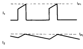
Fig. 33 Primary and secondary current waveforms under the current limiting operation condition on feed forward system
