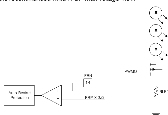
Figure 6 Short current protections
