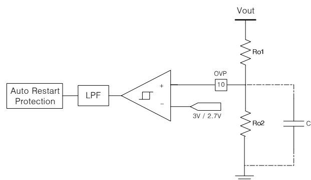
Figure 5 Over voltage protection circuit
