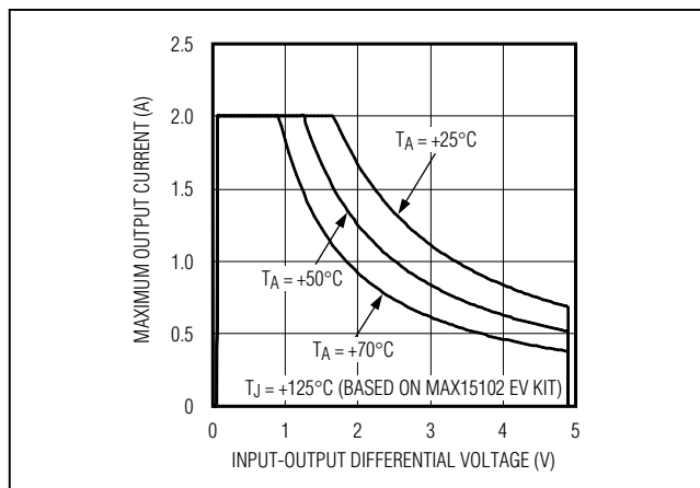
Figure 1. Maximum Output Current Curves
