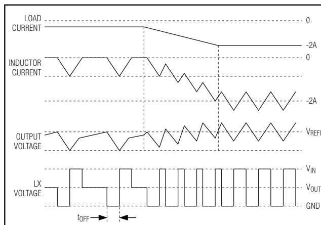
Figure 4. Sink-Mode Waveforms
