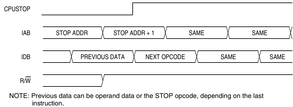
Figure 9-15. Stop Mode Entry Timing
