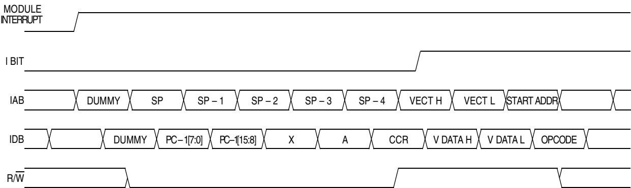
Figure 9-8. Interrupt Entry
