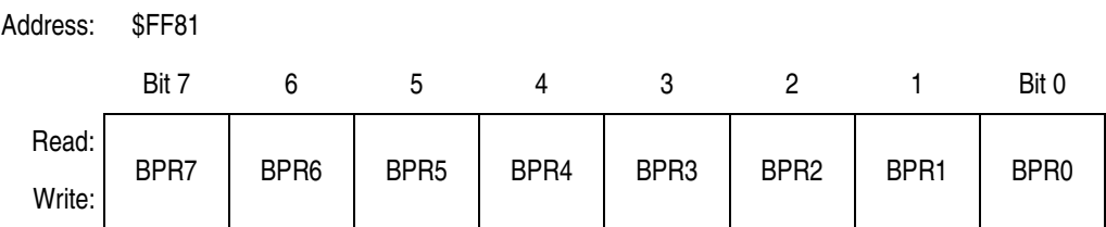
Figure 5-2. FLASH-2 Block Protect Register (FL2BPR)
