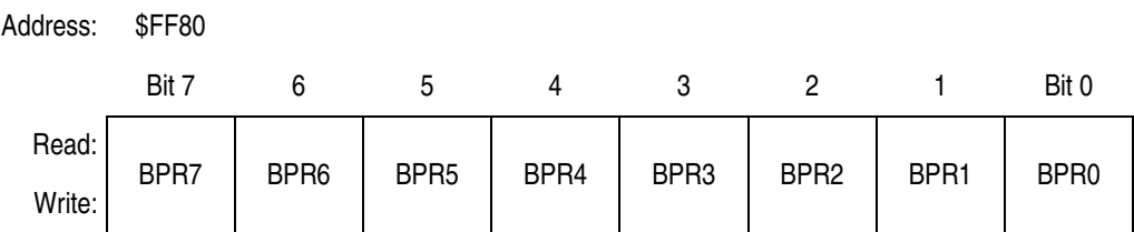
Figure 4-2. FLASH-1 Block Protect Register (FL1BPR)
