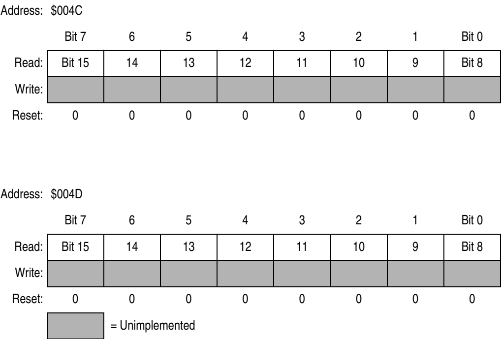
Figure 21-4. PIT Counter Registers (PCNTH–PCNTL)
