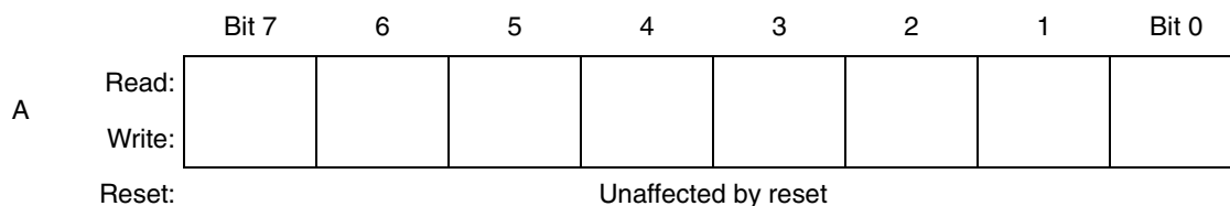
Figure 8-2. Accumulator (A)
