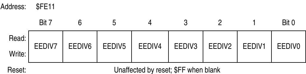
Figure 6-8. EEPROM-1 Divider Non-Volatile Register Low (EE1DIVLNVR)
