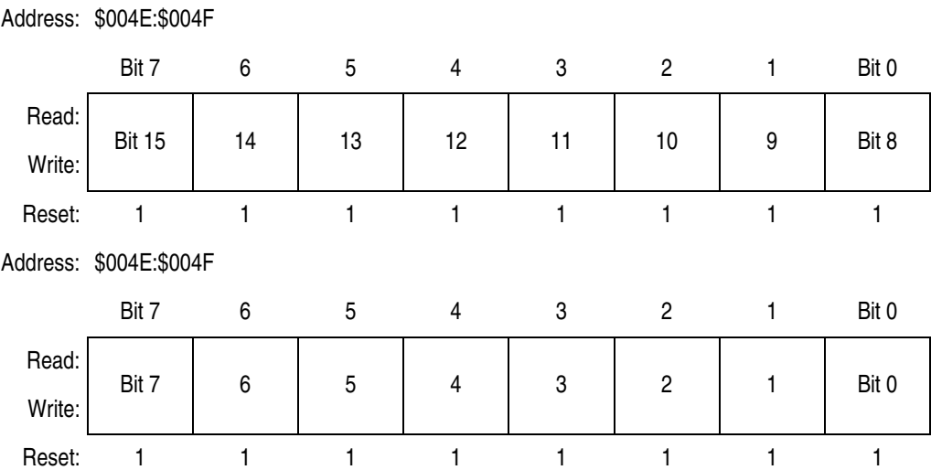
Figure 21-5. PIT Counter Modulo Registers (PMODH–PMODL)
