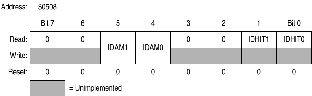
Figure 23-23. Identifier Acceptance Control Register (CIDAC)
