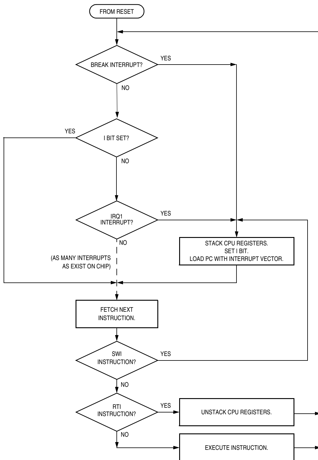
Figure 9-9. Interrupt Processing
