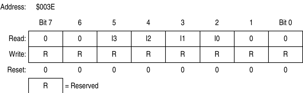
Figure 27-19. BDLC State Vector Register (BSVR)
