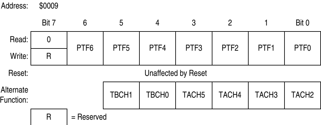
Figure 22-17. Port F Data Register (PTF)
