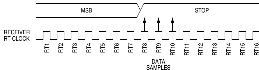
Figure 18-9. Slow Data
