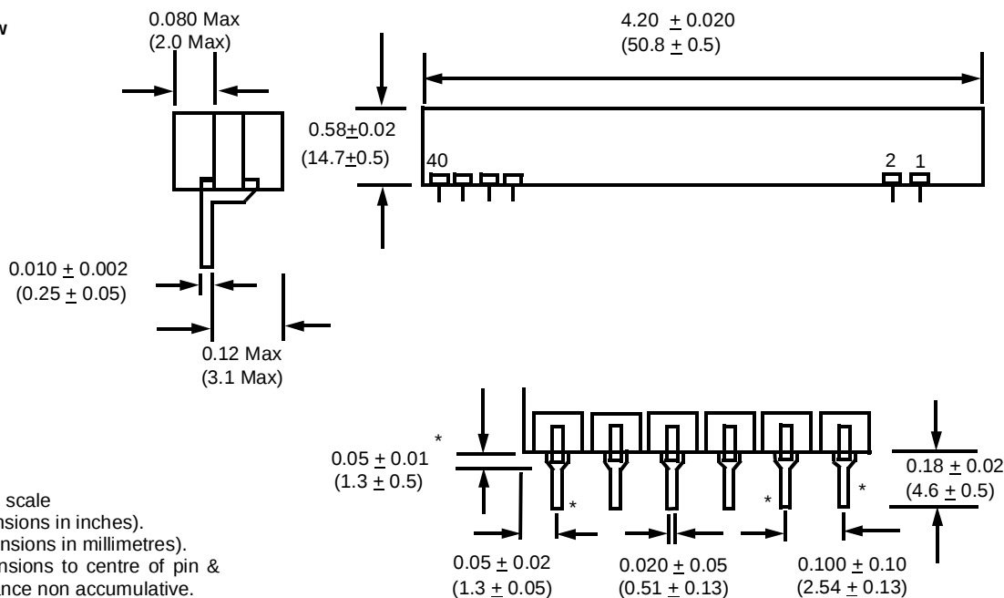
Figure 10 - Mechanical Data
