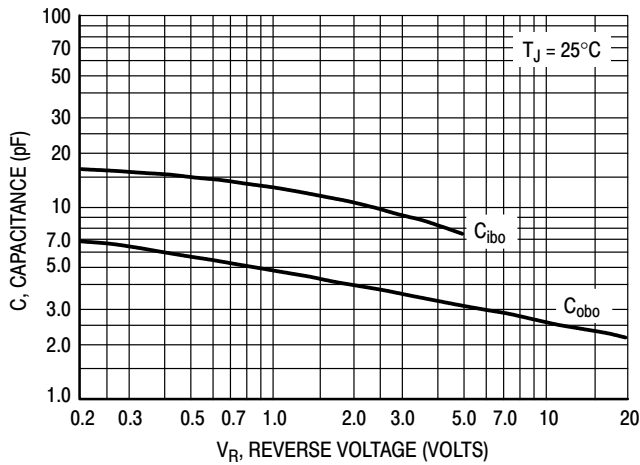
Figure 12. Capacitances
