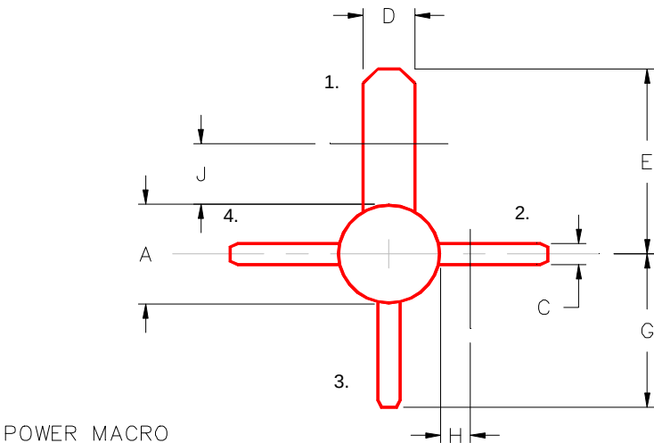
POWER MACRO
