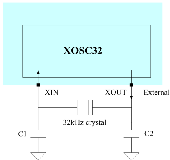
Figure 7. Block diagram of XOSC32
