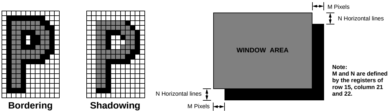
FIGURE 9. Character Bordering and Shadowing and Shadowing on Window
