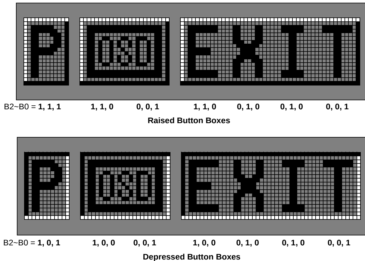
FIGURE 6. Character Button Boxes
