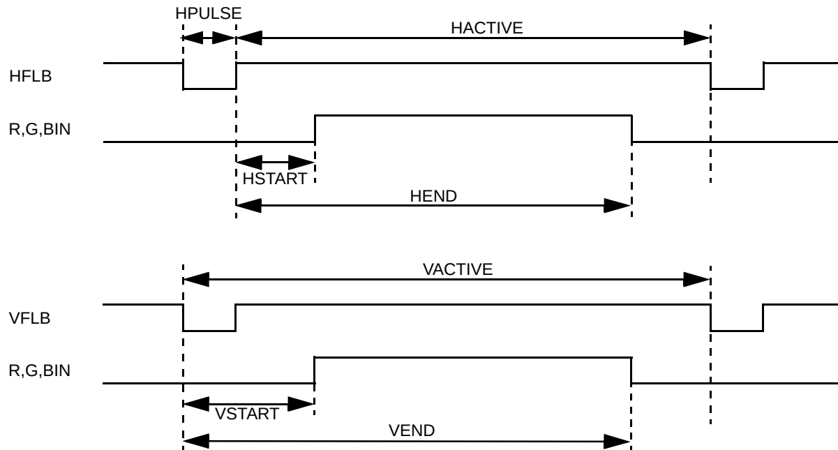
FIGURE 10. Timing Diagram of Auto Sizing Video Measurement
