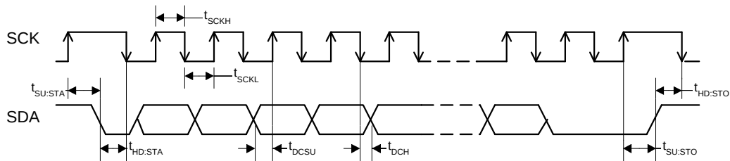
FIGURE 12. Data Interface Timing(I²C)
