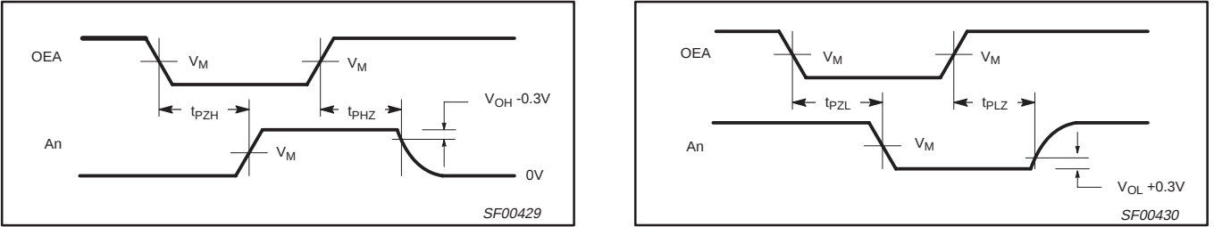
Waveform 3. 3-state output enable time to high level and output disable time from high level Waveform 4. 3-state output enable time to low level and output disable time from low level
