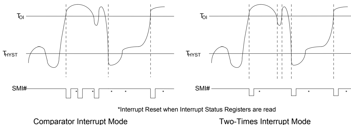
Figure 8-27 SMI Mode
