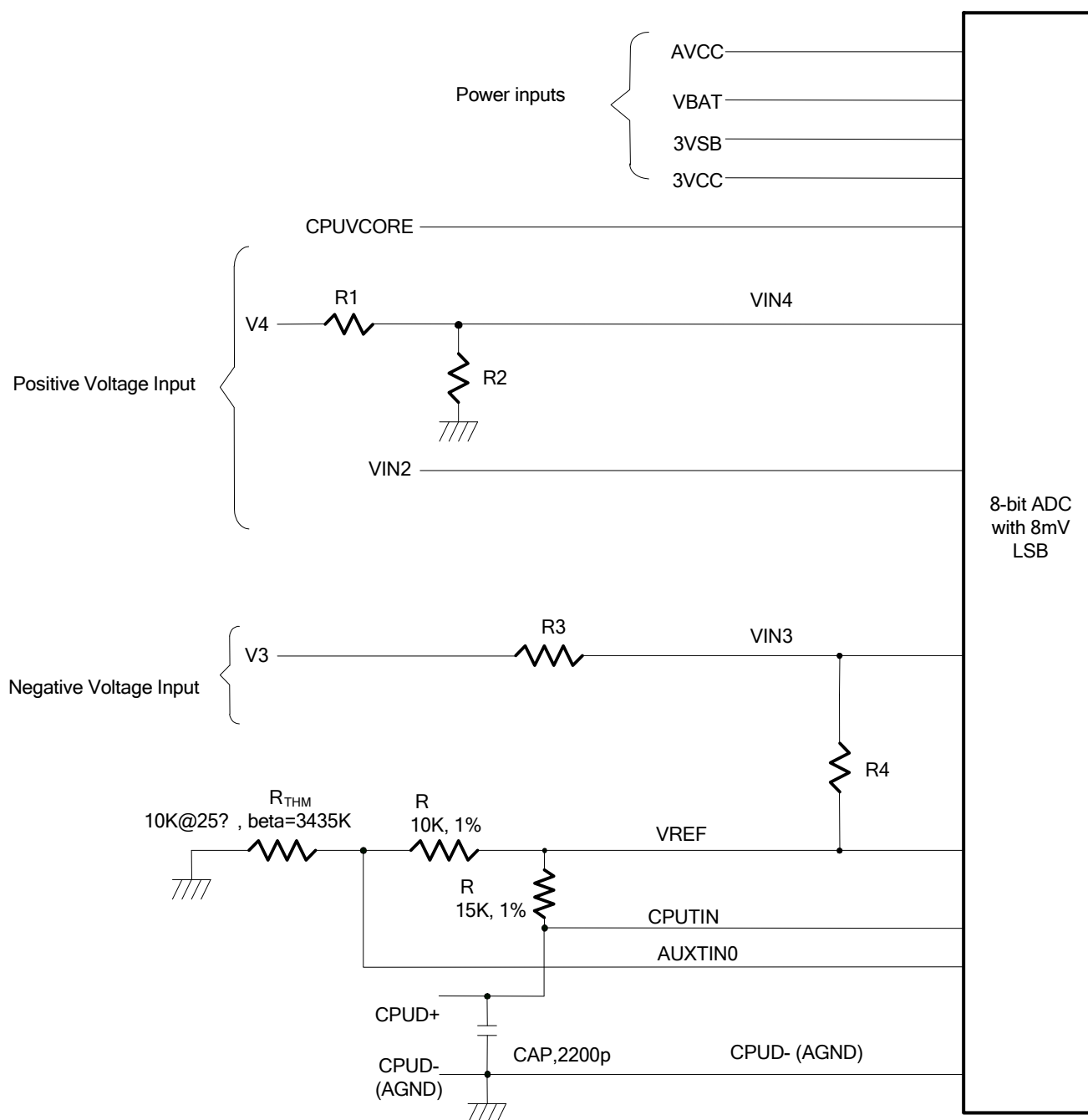
Figure 8-4 Analog Inputs and Application Circuit of the NCT5532D
