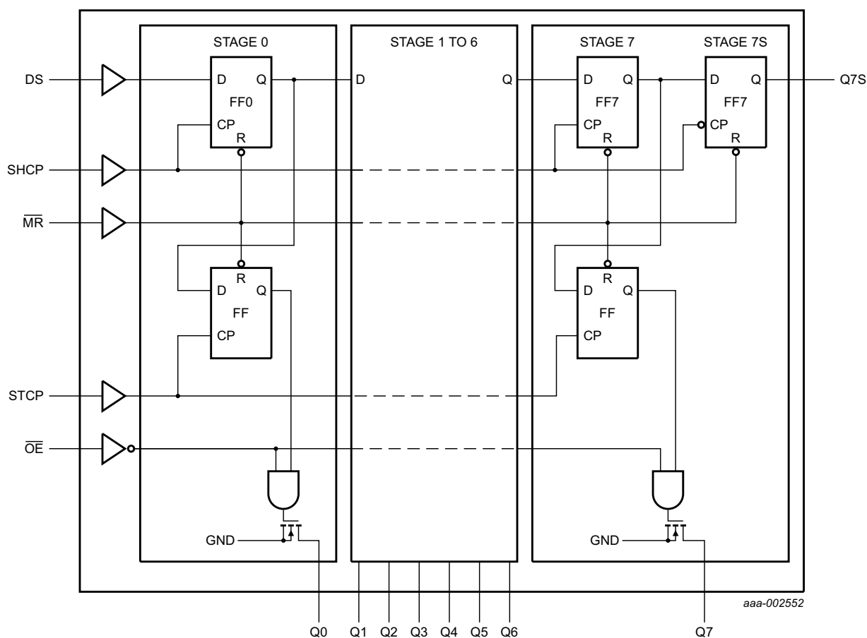
Fig 5. Logic diagram
