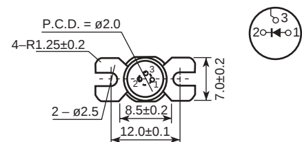
PIN CONNECTIONS
