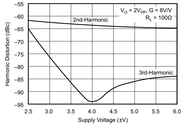
Figure 8. 10-MHz Harmonic Distortion vs Supply Voltage
