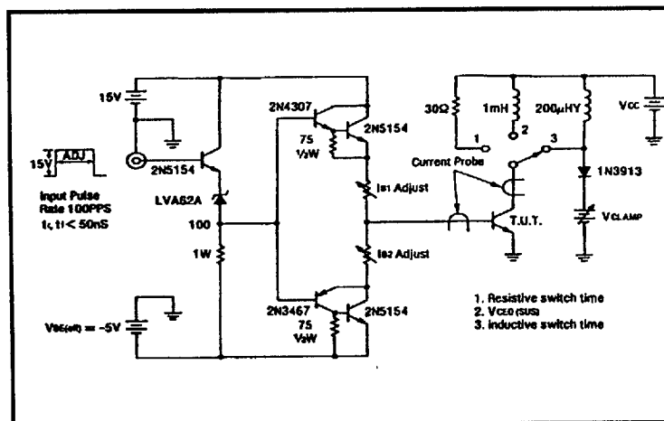
Switchtime Test Circuit
