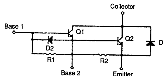
Schematic (Note 7)
