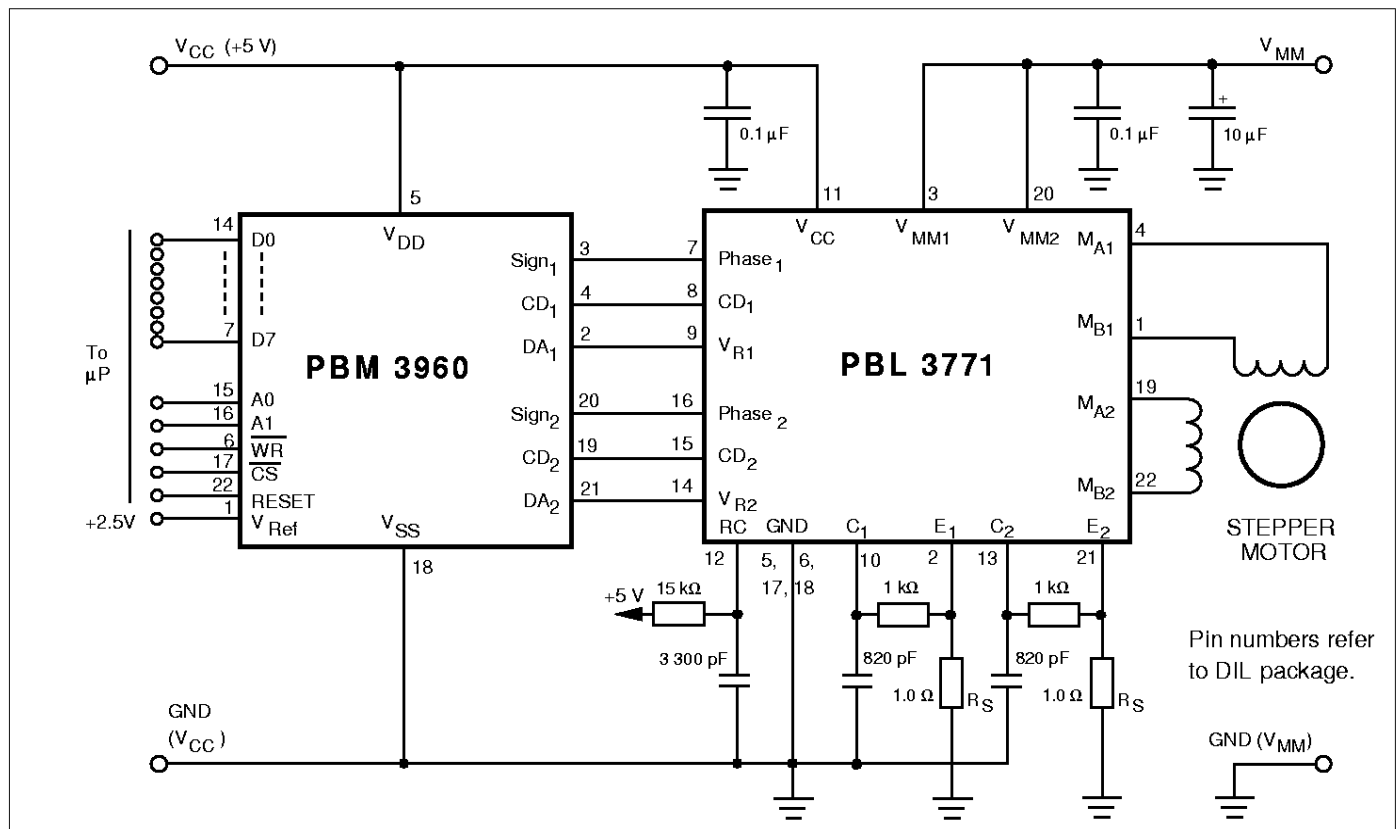
Figure 7. Microstepping system with PBM 3960 and PBL 3771.
