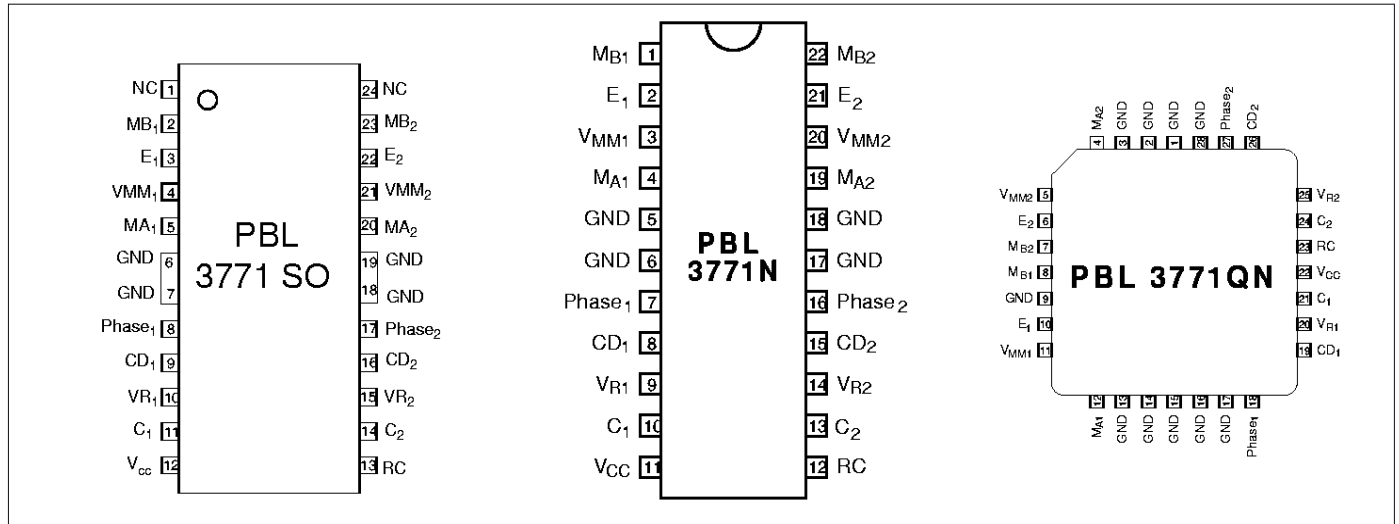
Figure 4. Pin configuration.
