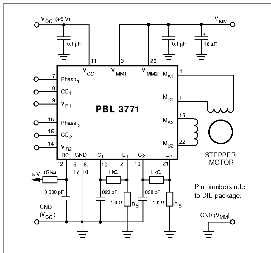
Figure 6. Typical stepper motor application with PBL 3771.
