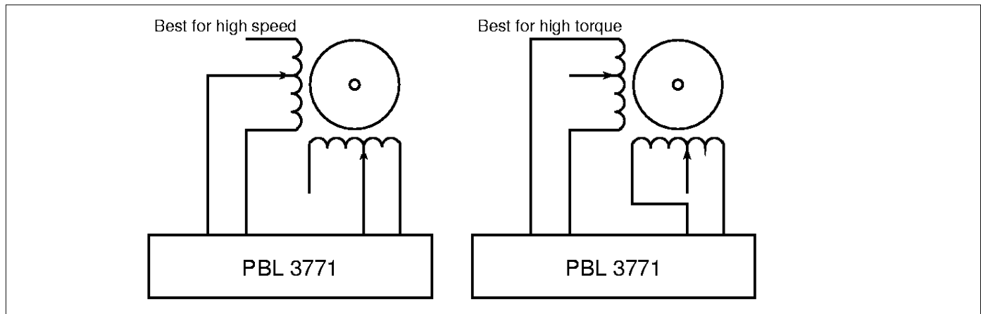
Figure 14. Connection of unipolar motors.
