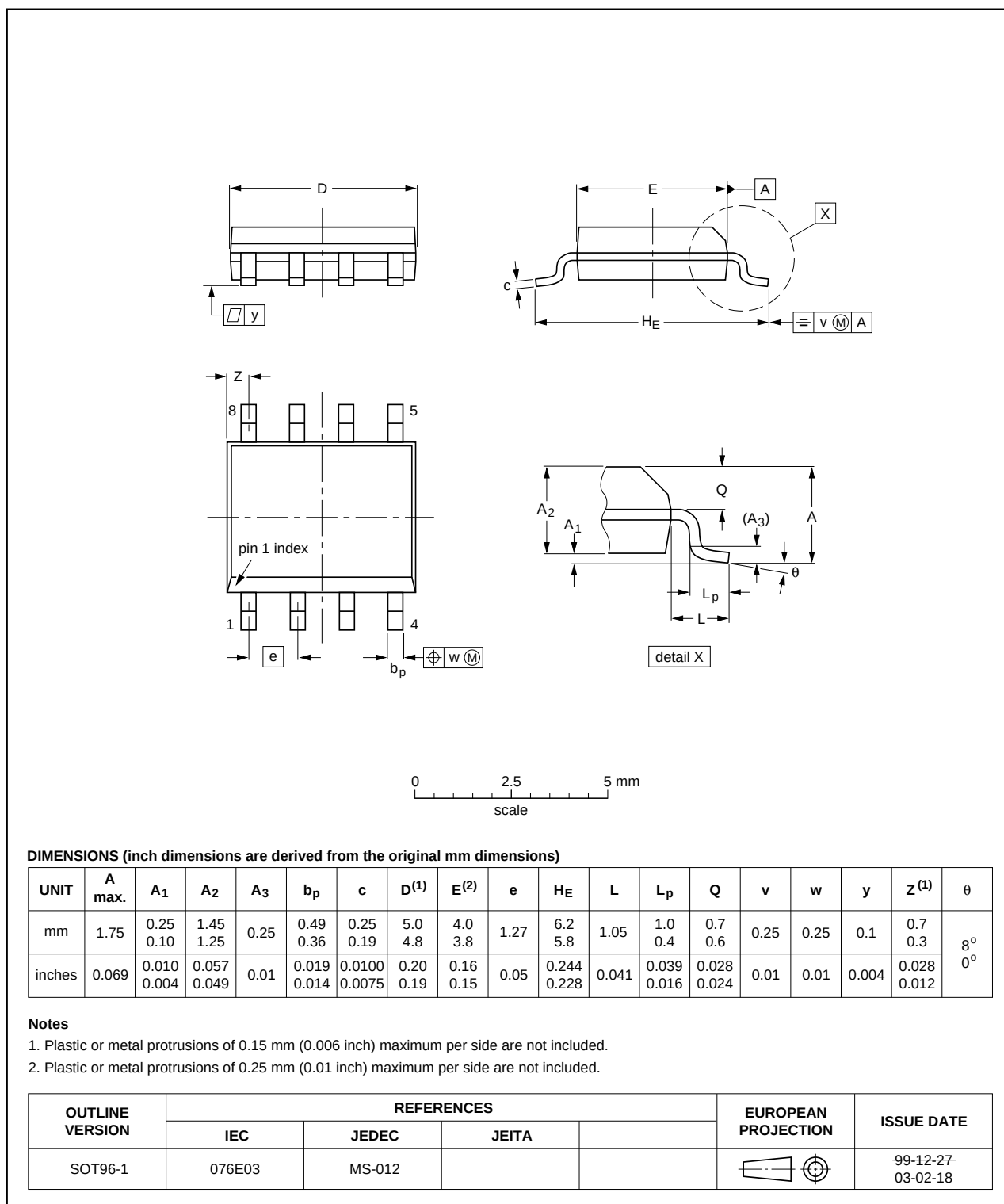
Fig 15. Package outline SOT96-1 (SO8)
