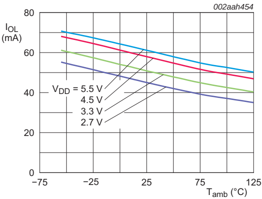
Fig 22. LOW-level output current on SDA pin versus temperature; V_{OL} = 0.4\text{ V}
