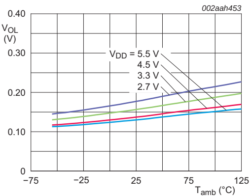
Fig 21. LOW-level output voltage on SDA pin versus temperature; I_{OL} = 20\text{ mA}
