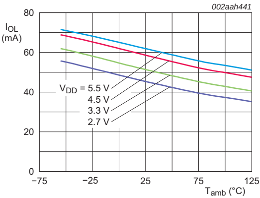
Fig 18. LOW-level output current on OS pin versus temperature; V_{OL} = 0.4 V
