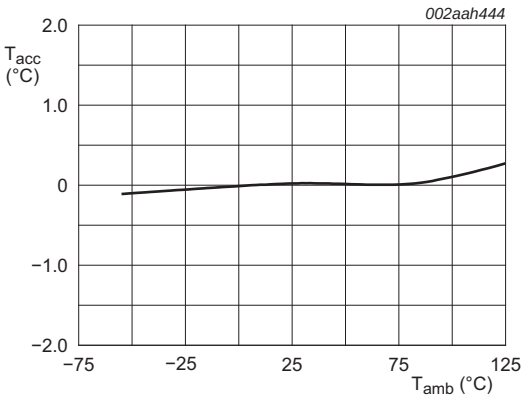
Fig 23. Temperature accuracy versus temperature; V_{CC} = 2.8\text{ V to }5.5\text{ V}
