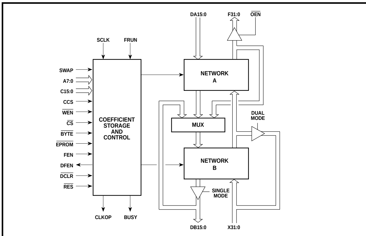
Figure. 4 Block Diagram
