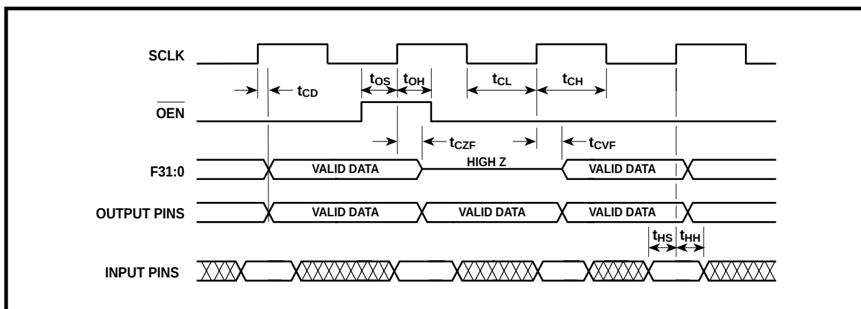
Figure. 22 Operating timings
