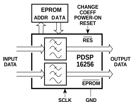
Figure. 1 A dual filter application
