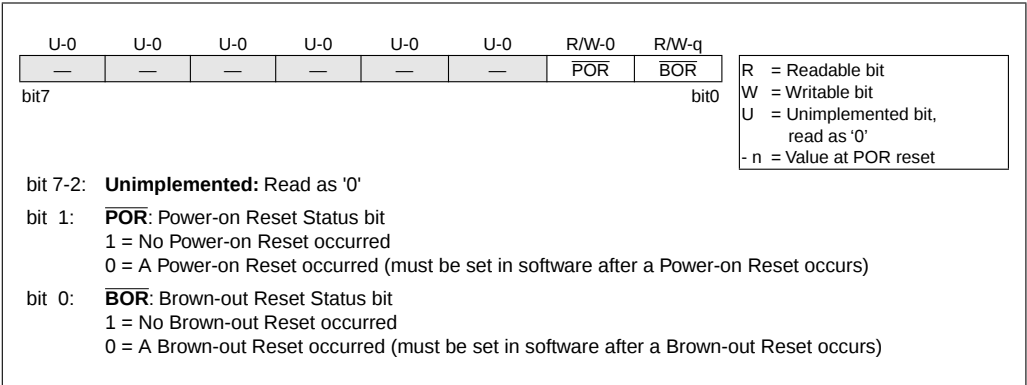
FIGURE 2-8: PCON REGISTER (ADDRESS 8Eh)
