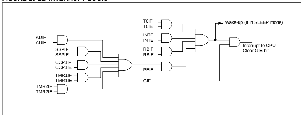
FIGURE 10-11: INTERRUPT LOGIC
