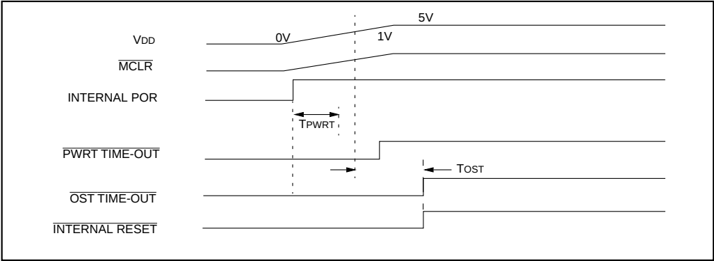
FIGURE 10-10: SLOW RISE TIME ( \overline{\text{MCLR}} TIED TO V_{DD} )
