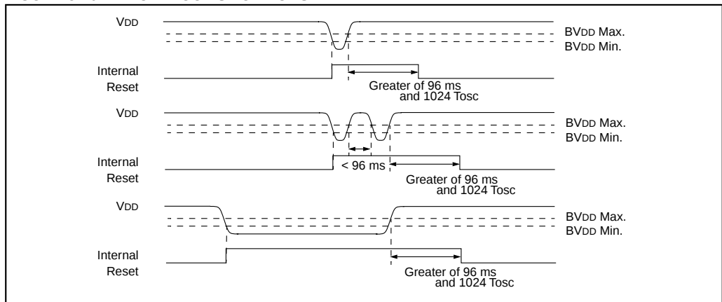
FIGURE 5-10: BROWN-OUT SITUATIONS
