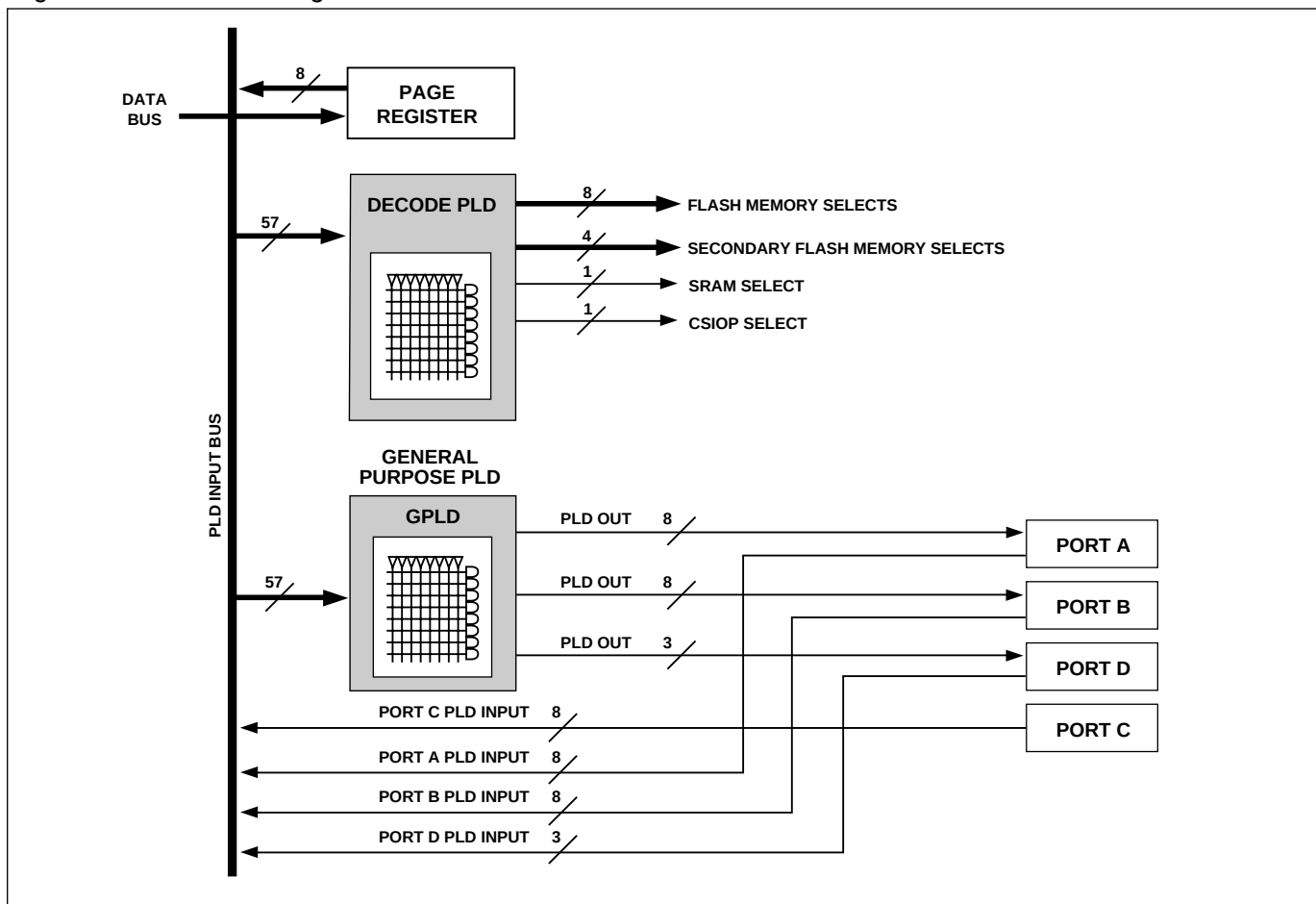
Figure 9. PLD Block Diagrams
