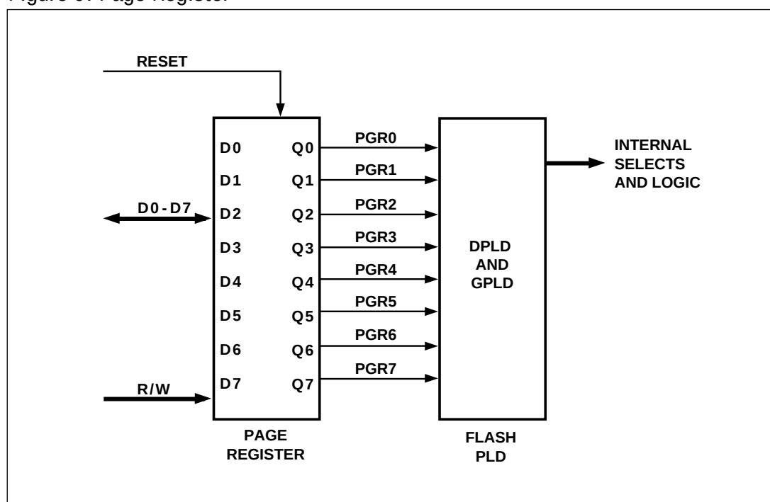
Figure 9. Page Register
