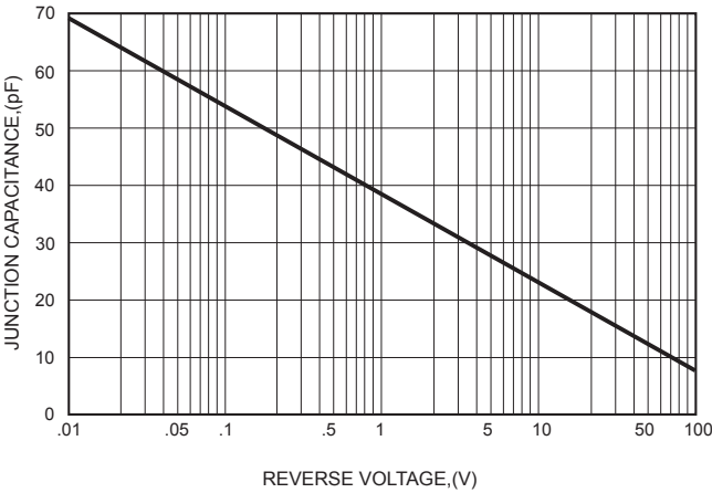
FIG.4-TYPICAL JUNCTION CAPACITANCE
