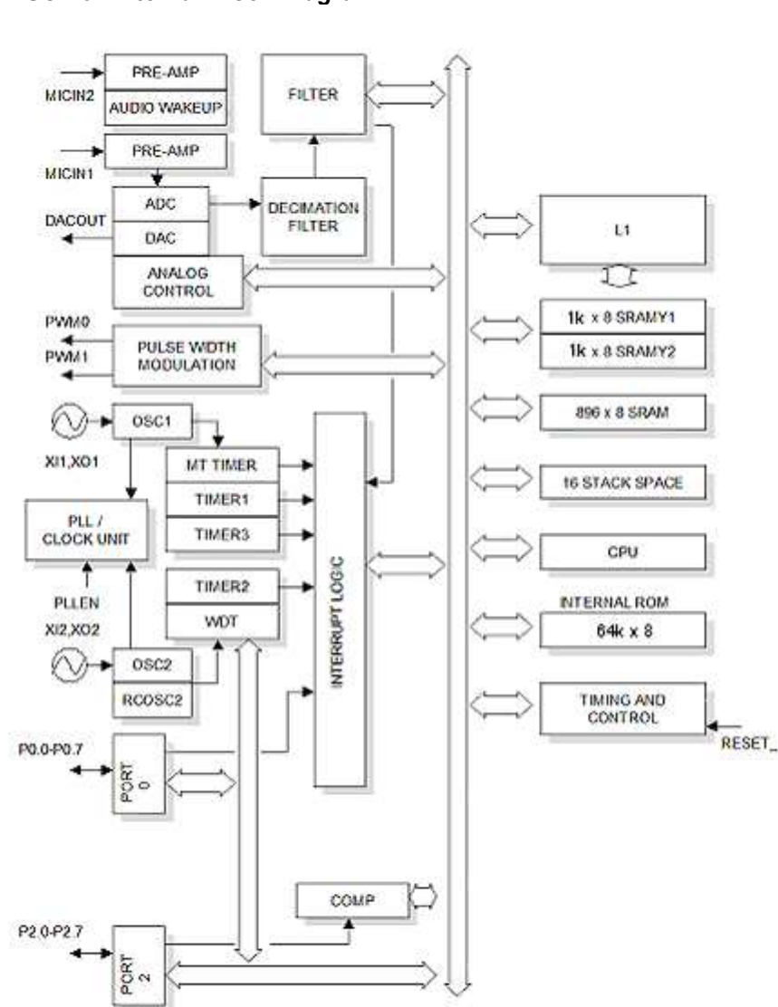
RSC-464 Internal Block Diagram
