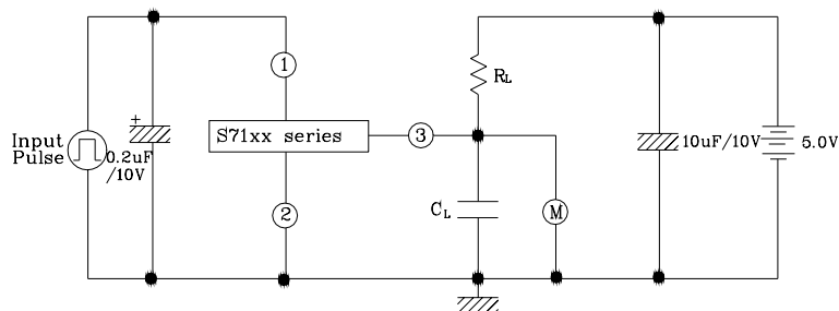
Test Circuit 2
